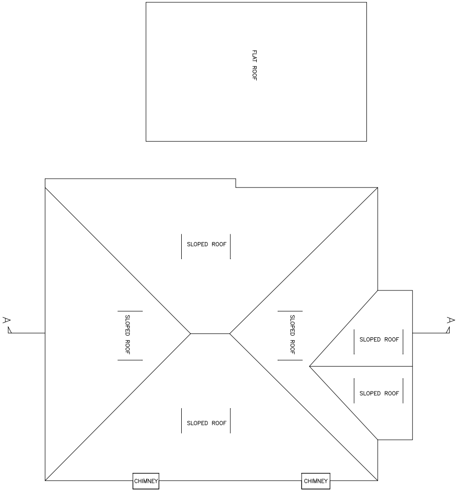
ROOF PLAN
