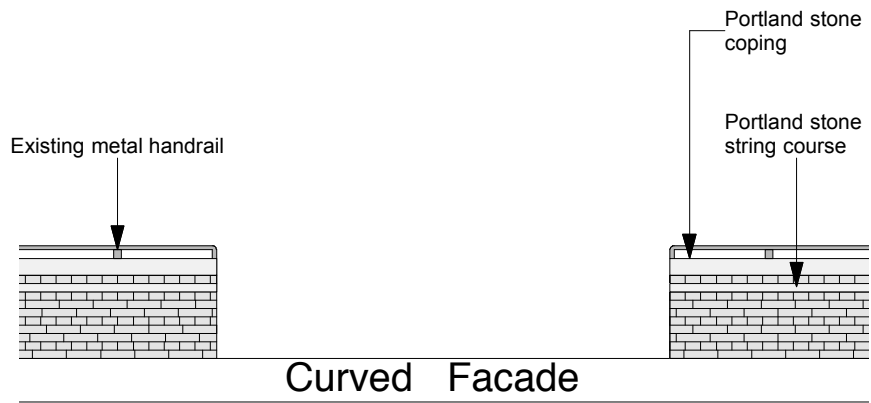
Detail 1 - Existing Moat Elevation @ 1:50
