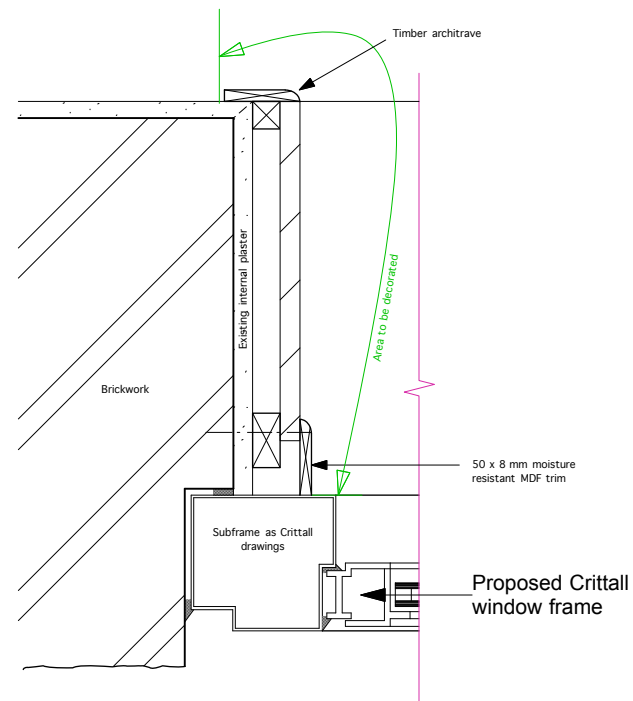
Detail 2 - Proposed Boarded Reveal
