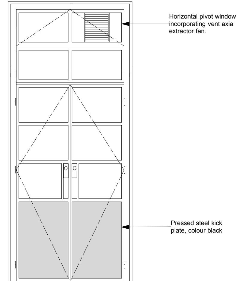
Detail 3 - Proposed New Door @ 1:25
