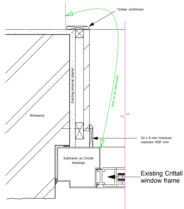
Detail 2 - Existing Boarded Reveal
