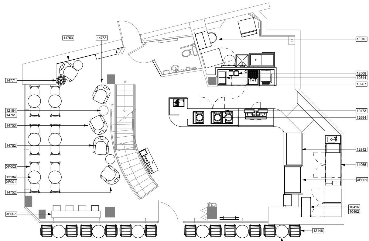
2 GROUND FLOOR - FURNITURE, FIXTURES, AND EQUIPMENT PLAN Scale: 1 : 50
