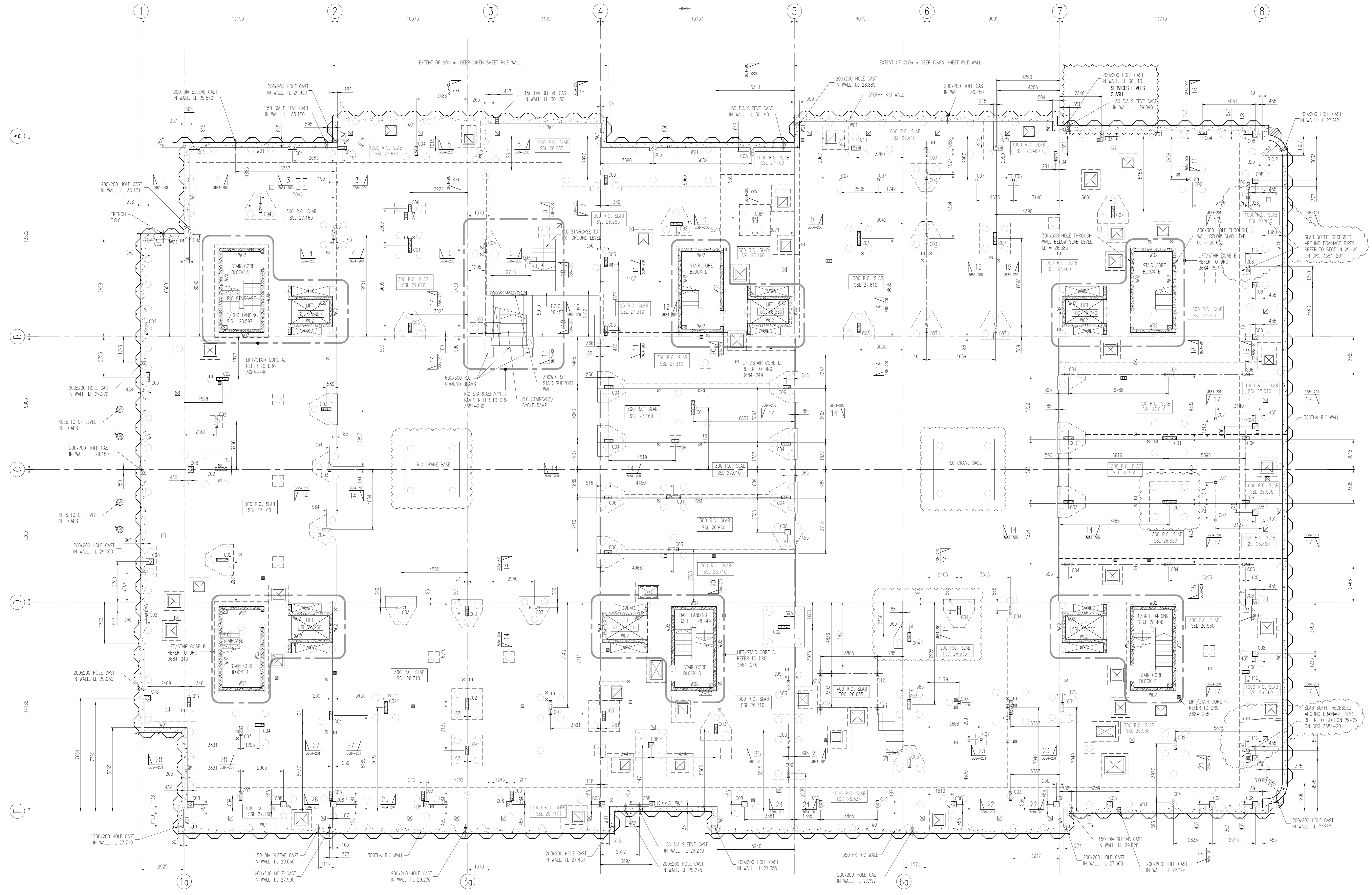
LOWER GROUND FLOOR PLAN 1:100
