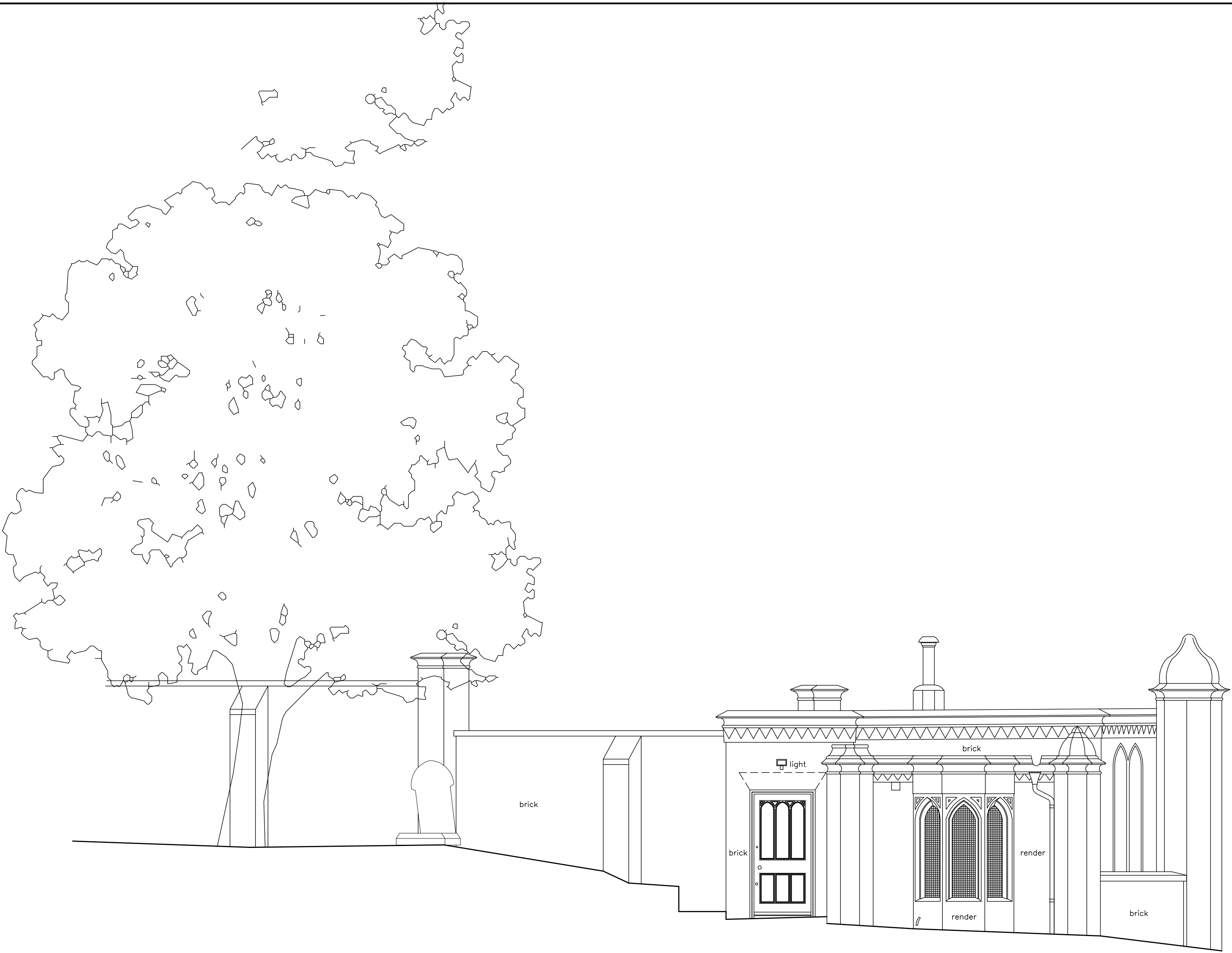
ELEVATION B - B (True View) 87.00m A.O.D.
