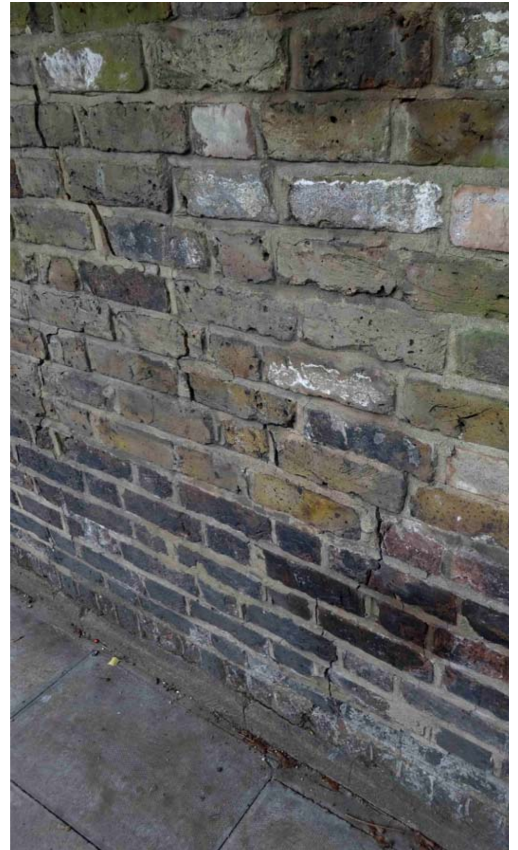
VIEW FROM PAVEMENT TOWARDS BASE OF WALL SHOWING ANGLE OF LEAN AND CRACKING
