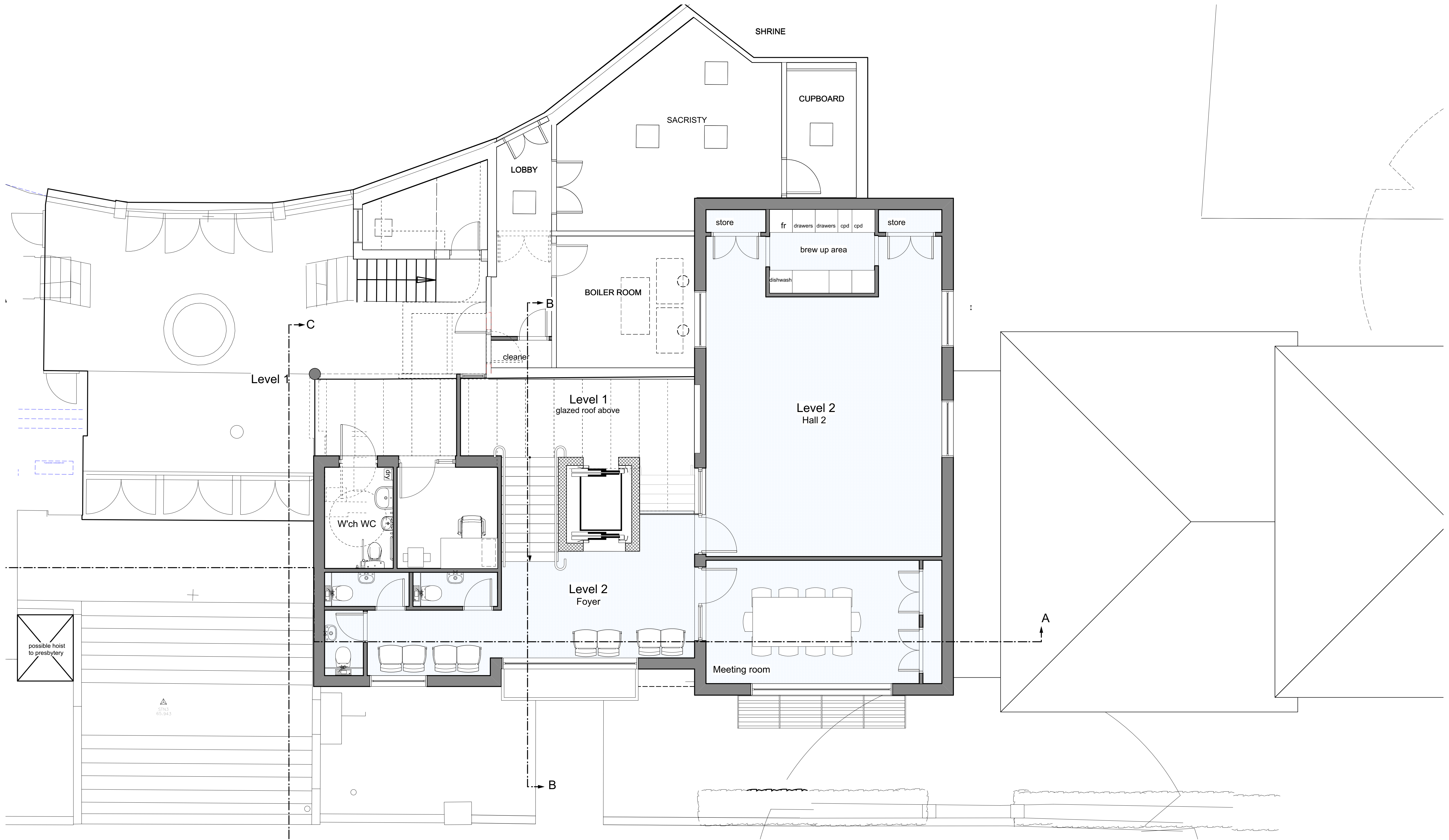
Proposed First Floor
