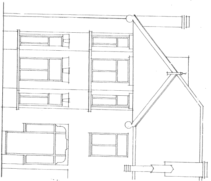
Front Elevation
