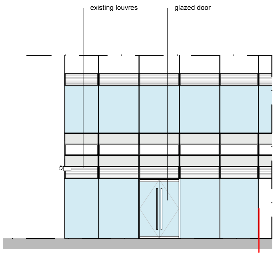
02 WEST ELEVATION - EXISTING
