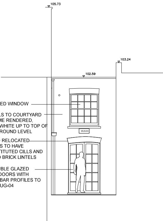
PROPOSED ELEVATION 1
