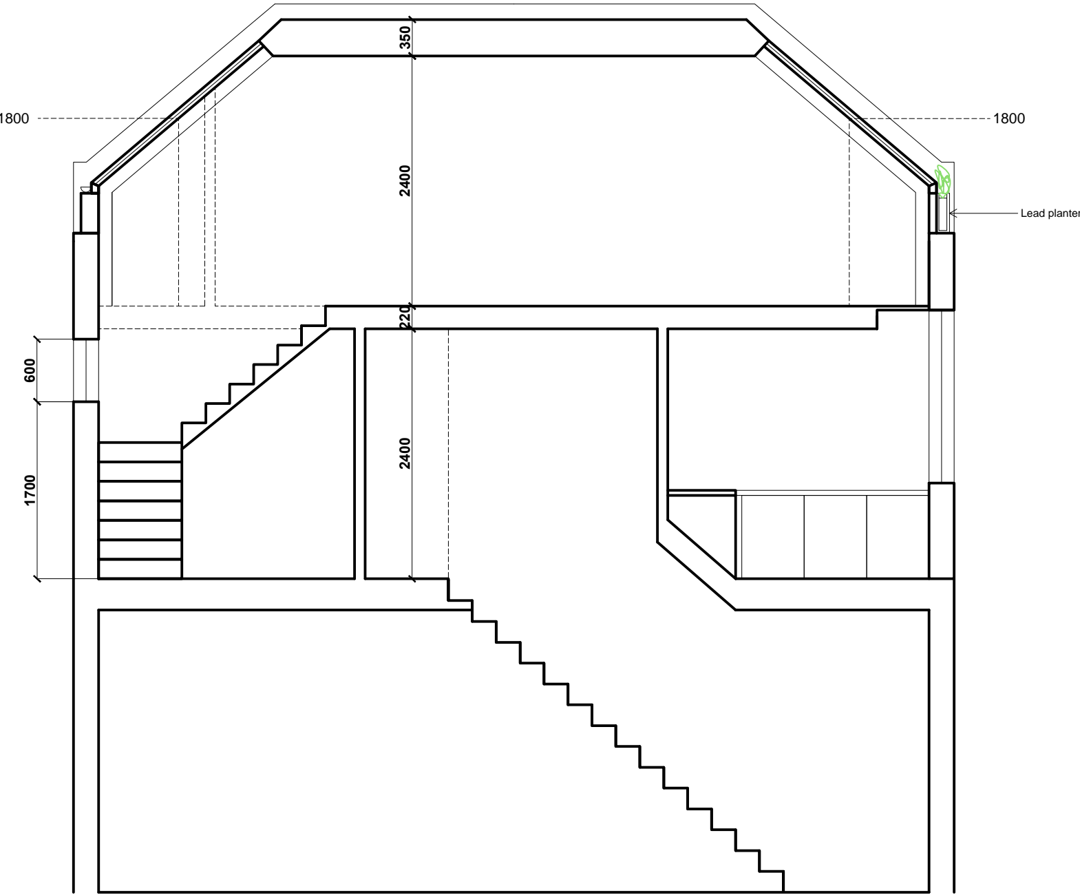
Proposed Section BB
