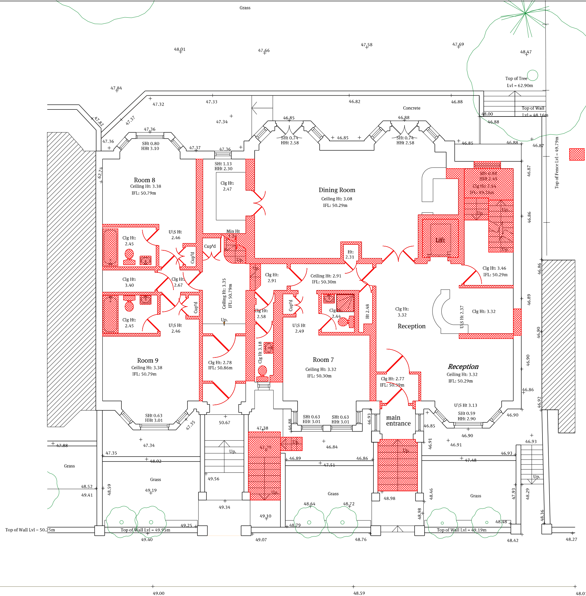
01 Existing Ground Floor Plan 1:100@A3
