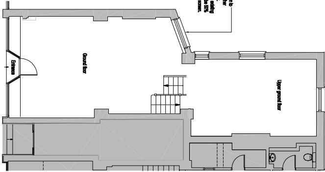
Ground Floor Plan 1:100
