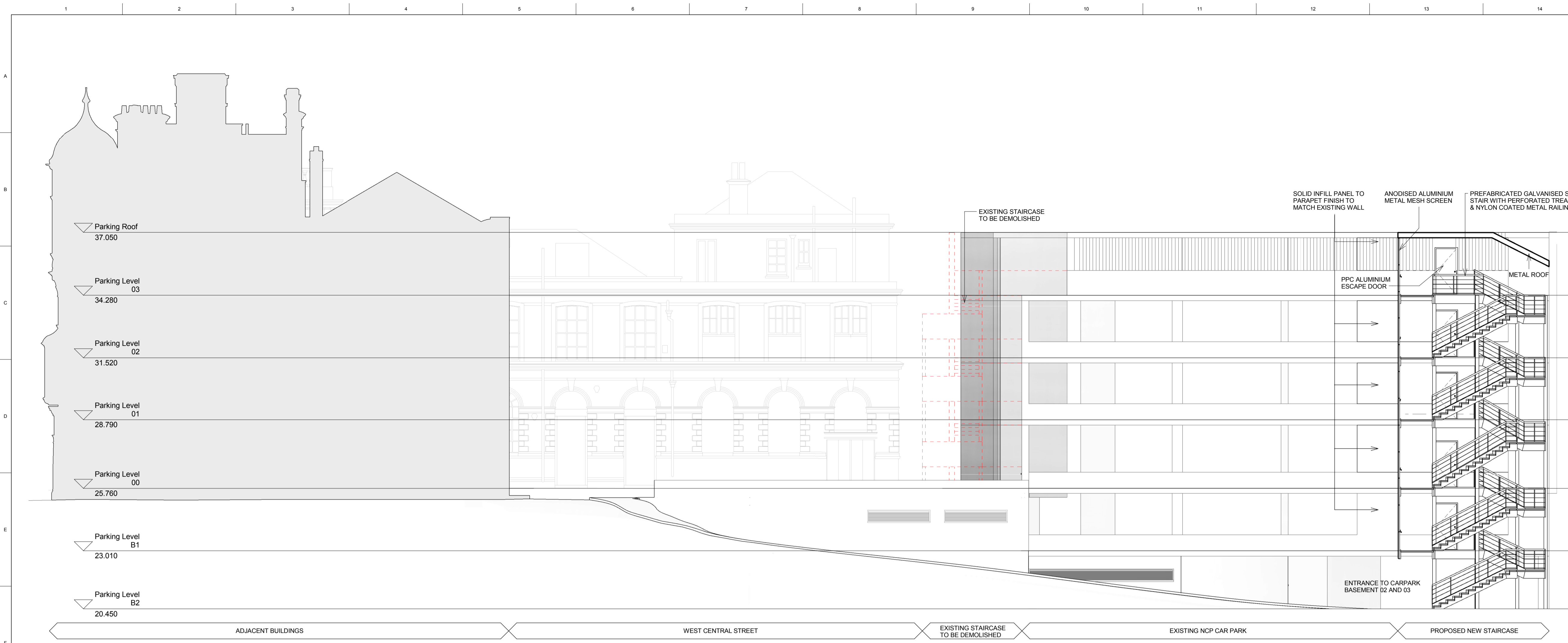
1 ELEVATION A 1:100
