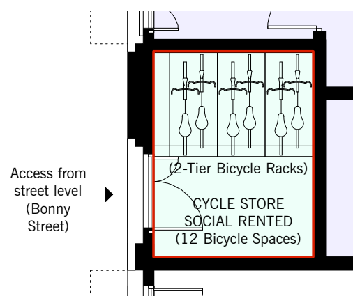
CYCLE STORAGE SOCIAL RENTED (STREET LEVEL)
