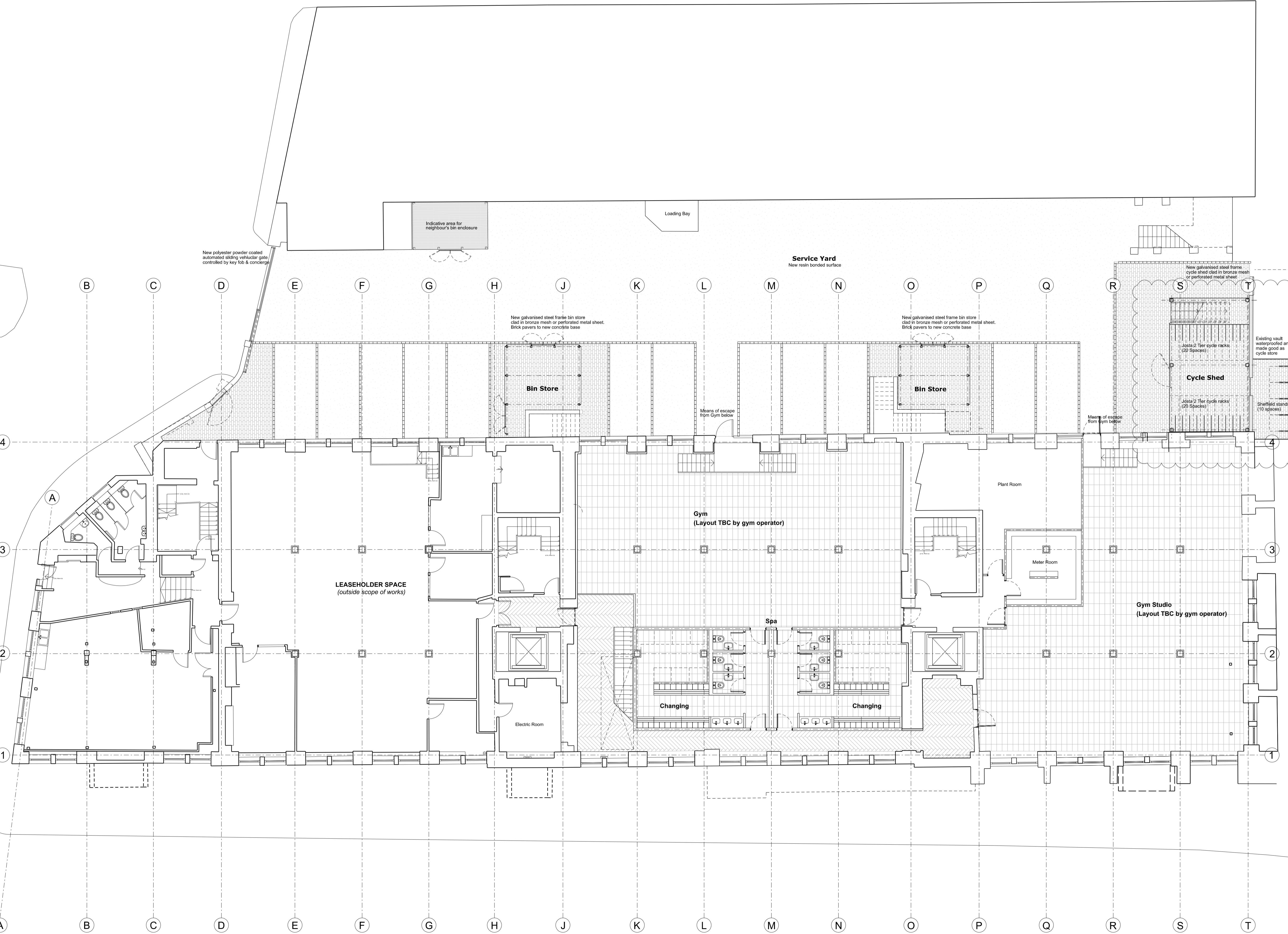
1 Basement as proposed 152_119 Scale 1:100 @ A1
