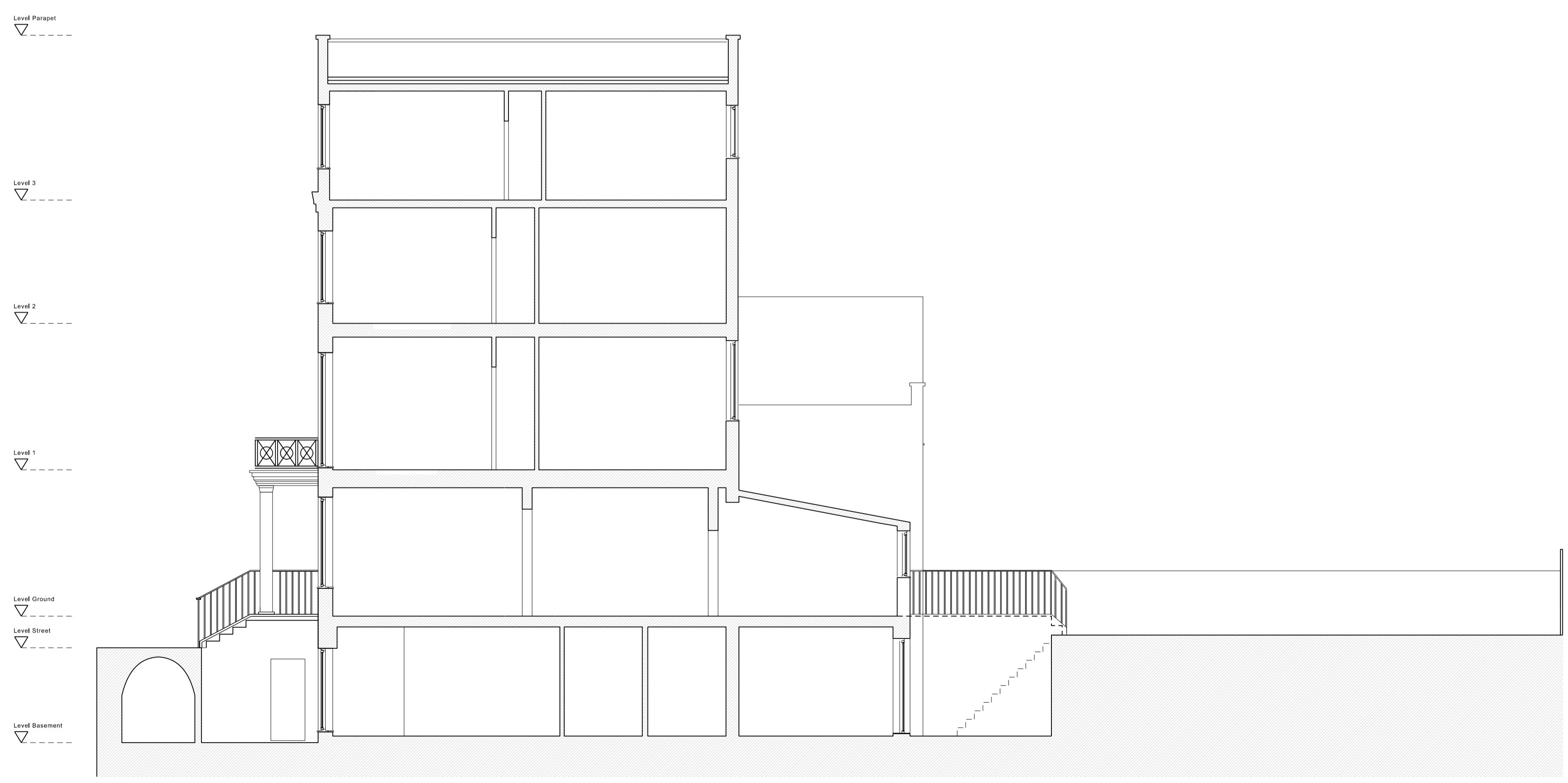
01 SECTION AA Proposed / Scale 1:50
