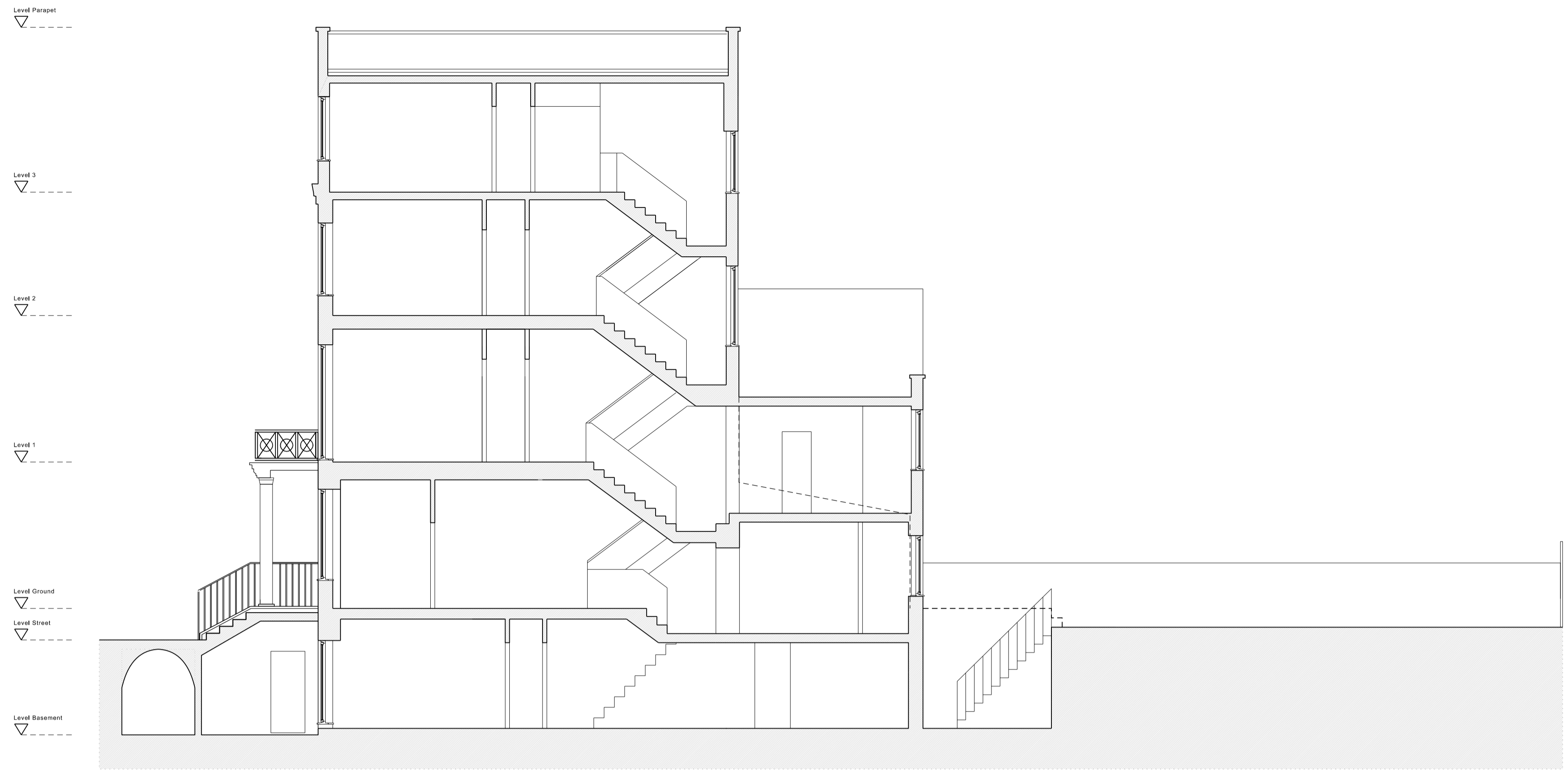
01 SECTION AA Proposed / Scale 1:50
