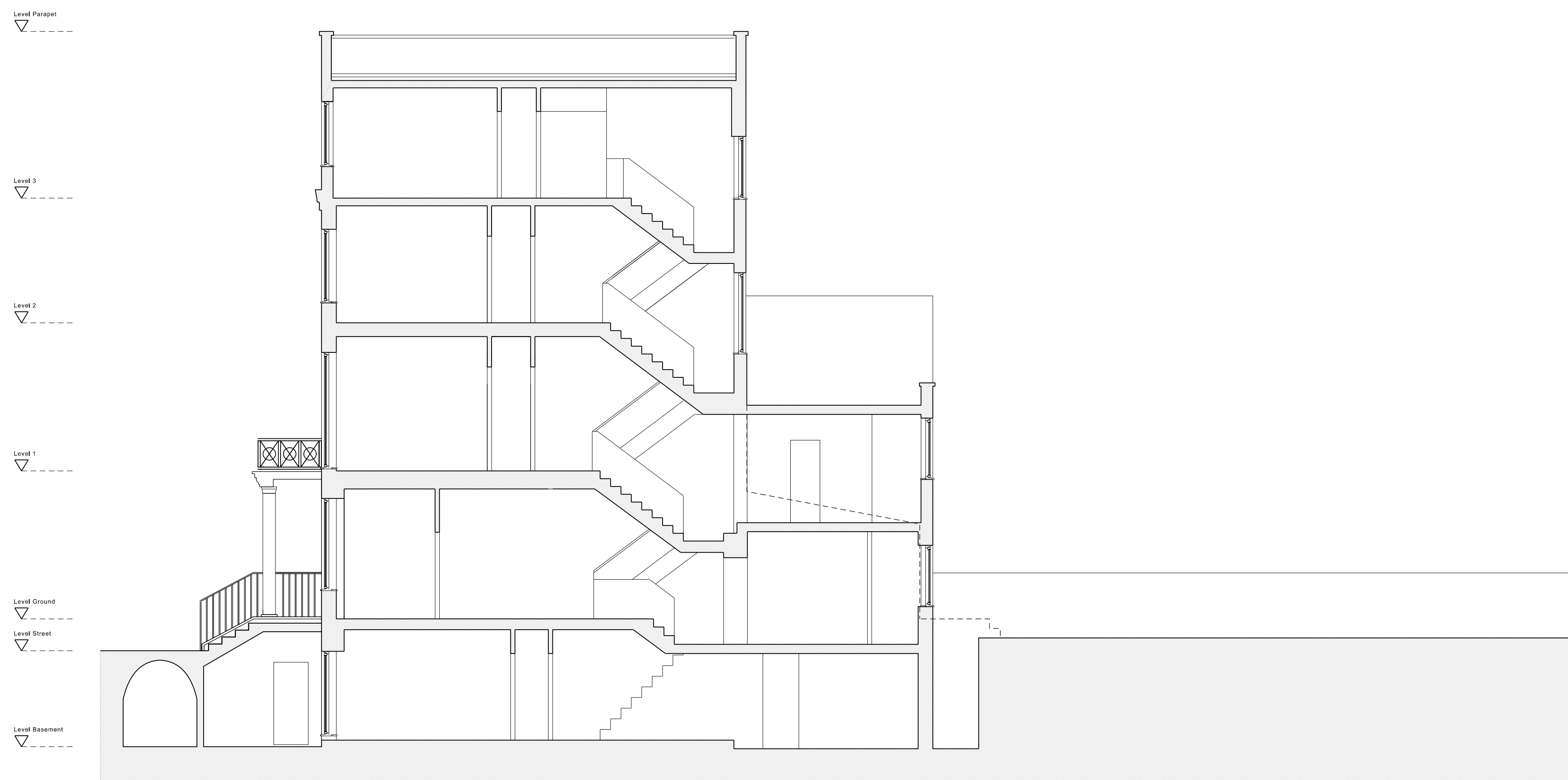
01 SECTION AA Existing / Scale 1:50
