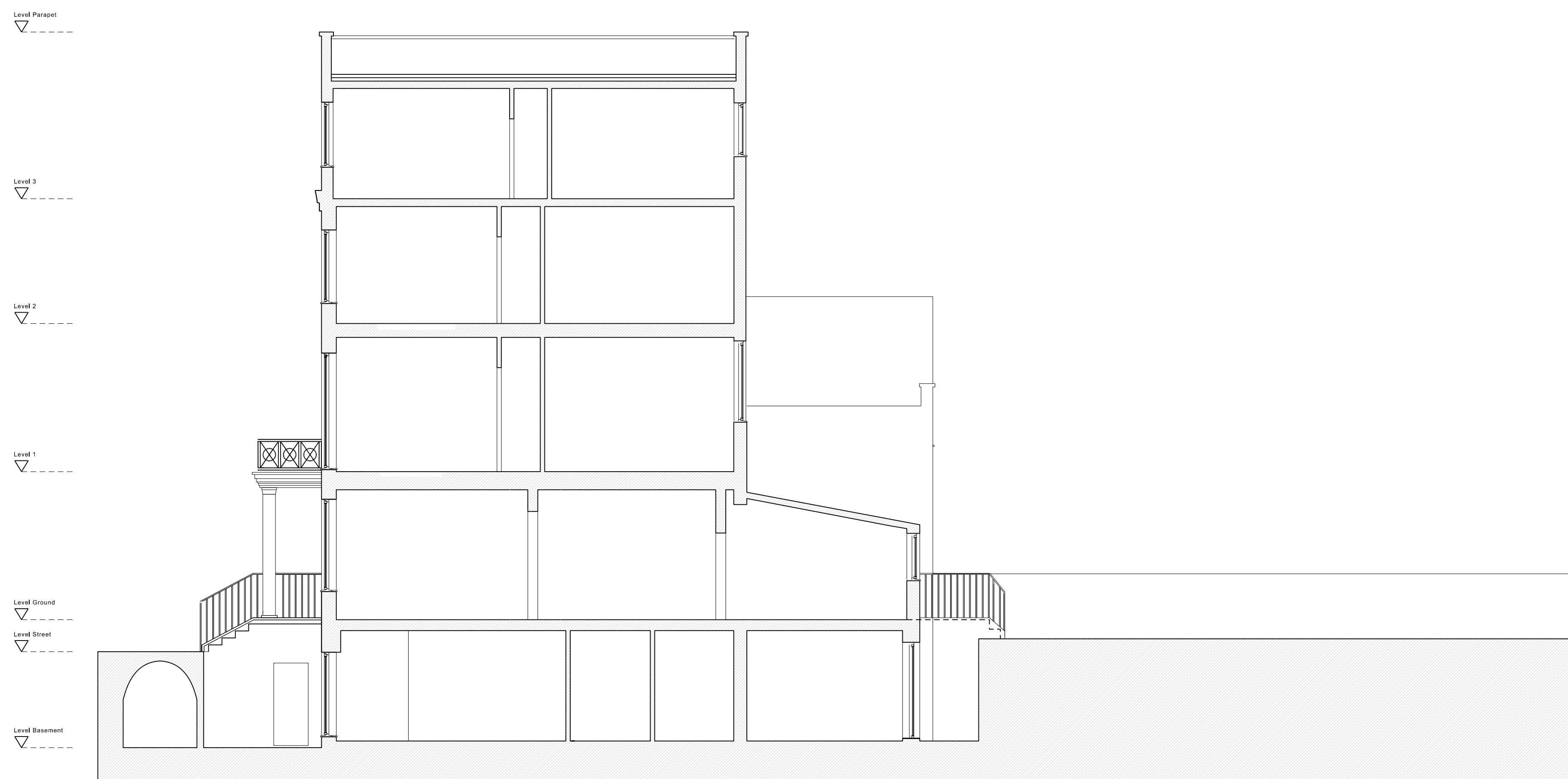
01 SECTION AA Existing / Scale 1:50
