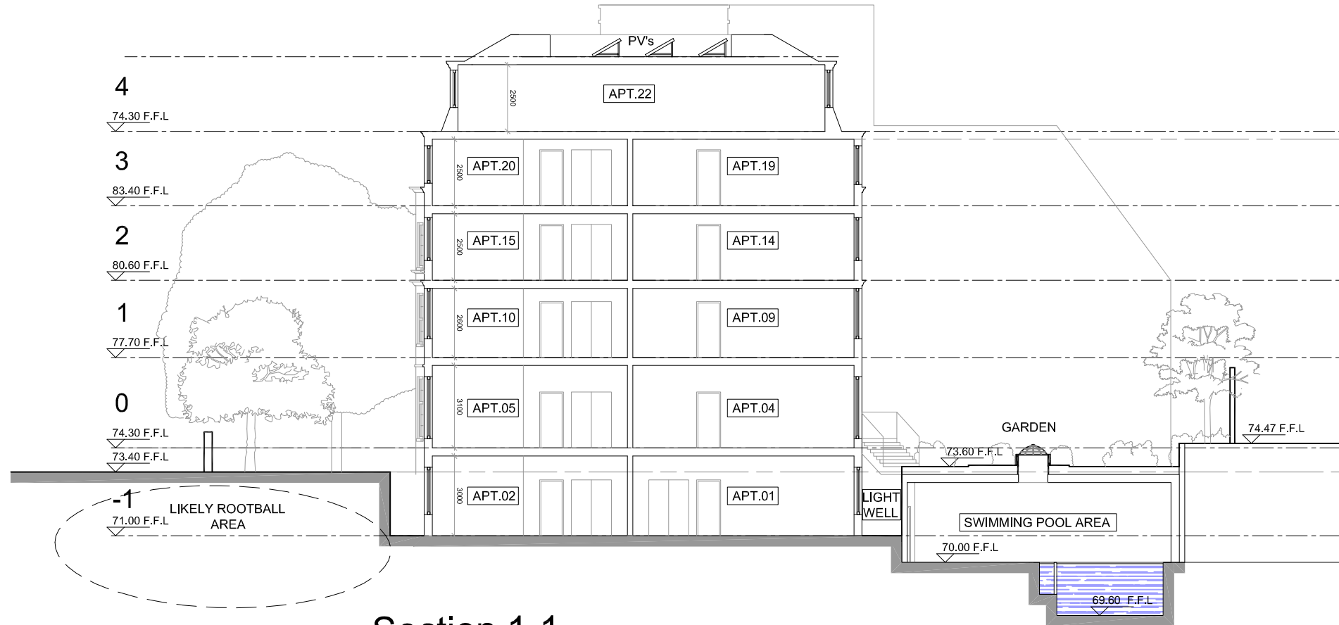
Section 1-1
