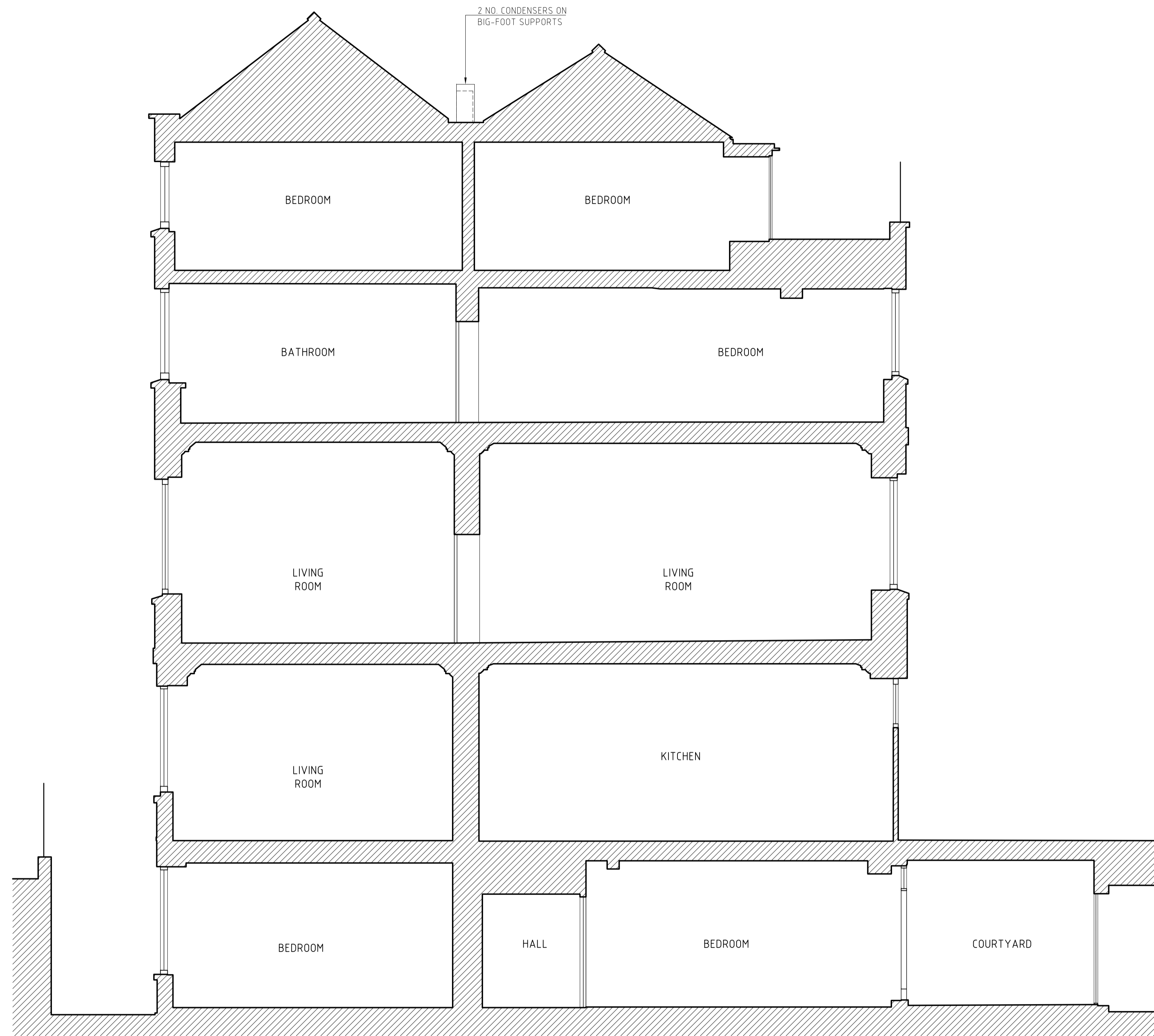
01 SECTION AA (01)810 As Proposed
