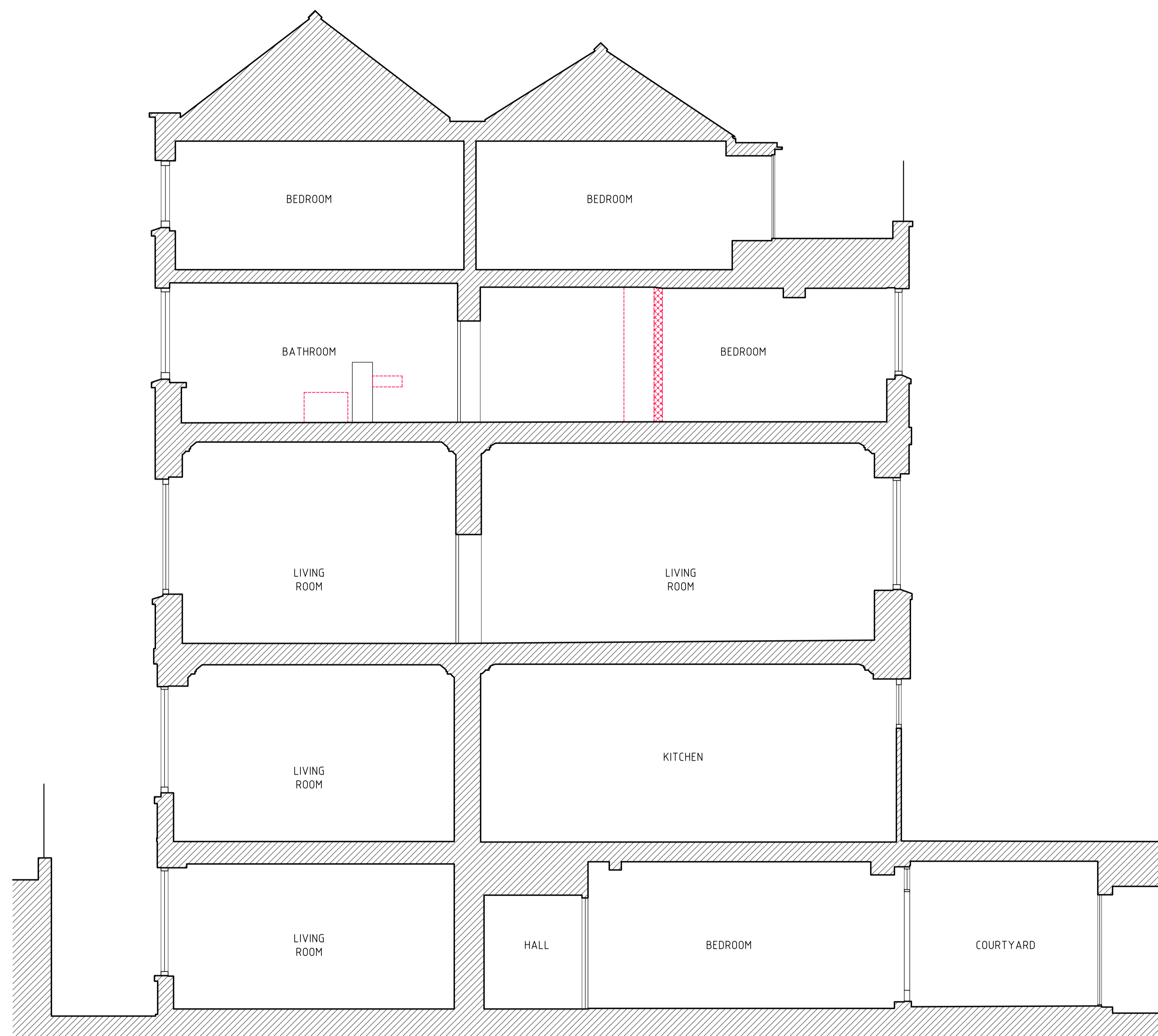
01 SECTION AA (01)310 As Existing with Demolitions
