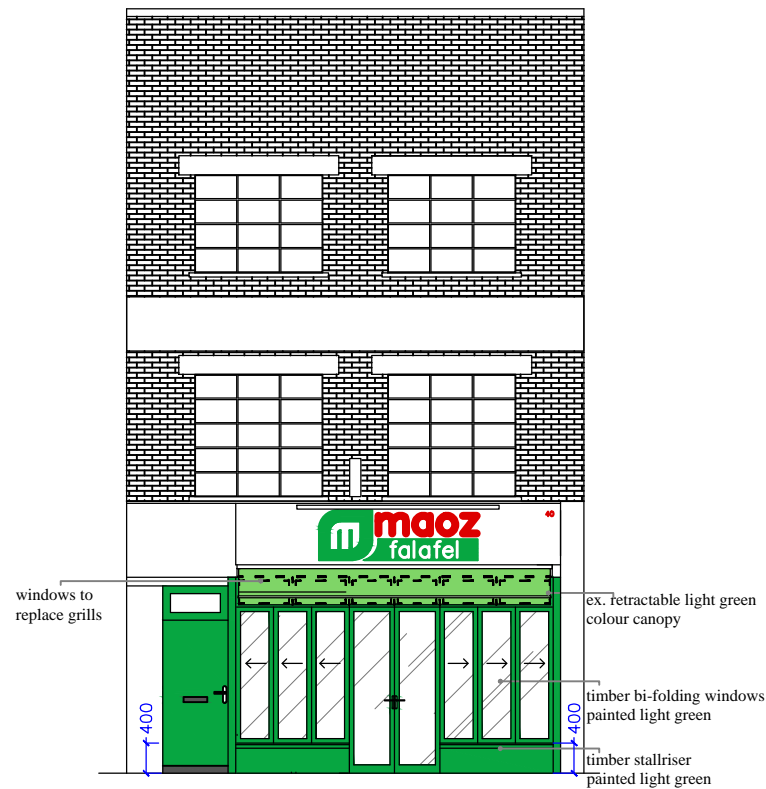
FRONT ELEVATION (as proposed)
