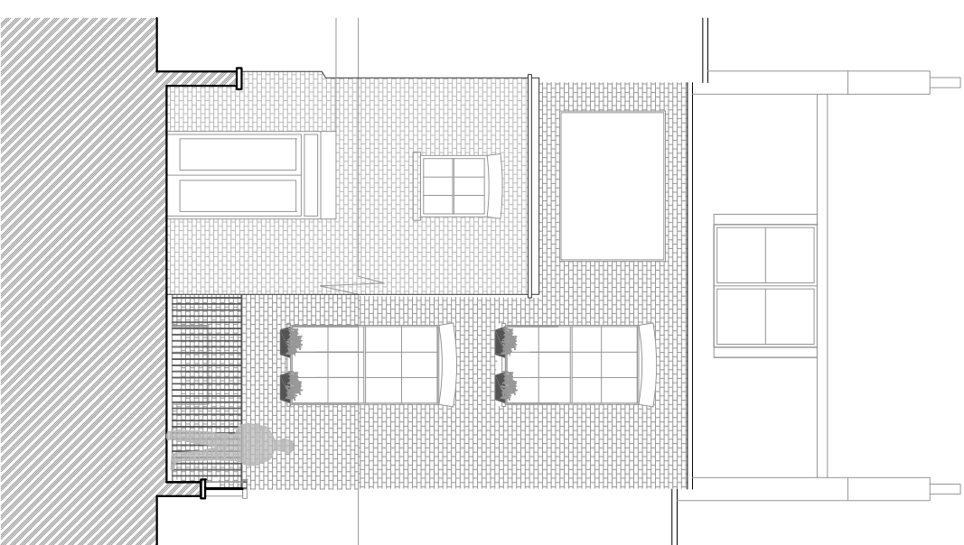
REAR ELEVATION E: 1/100
