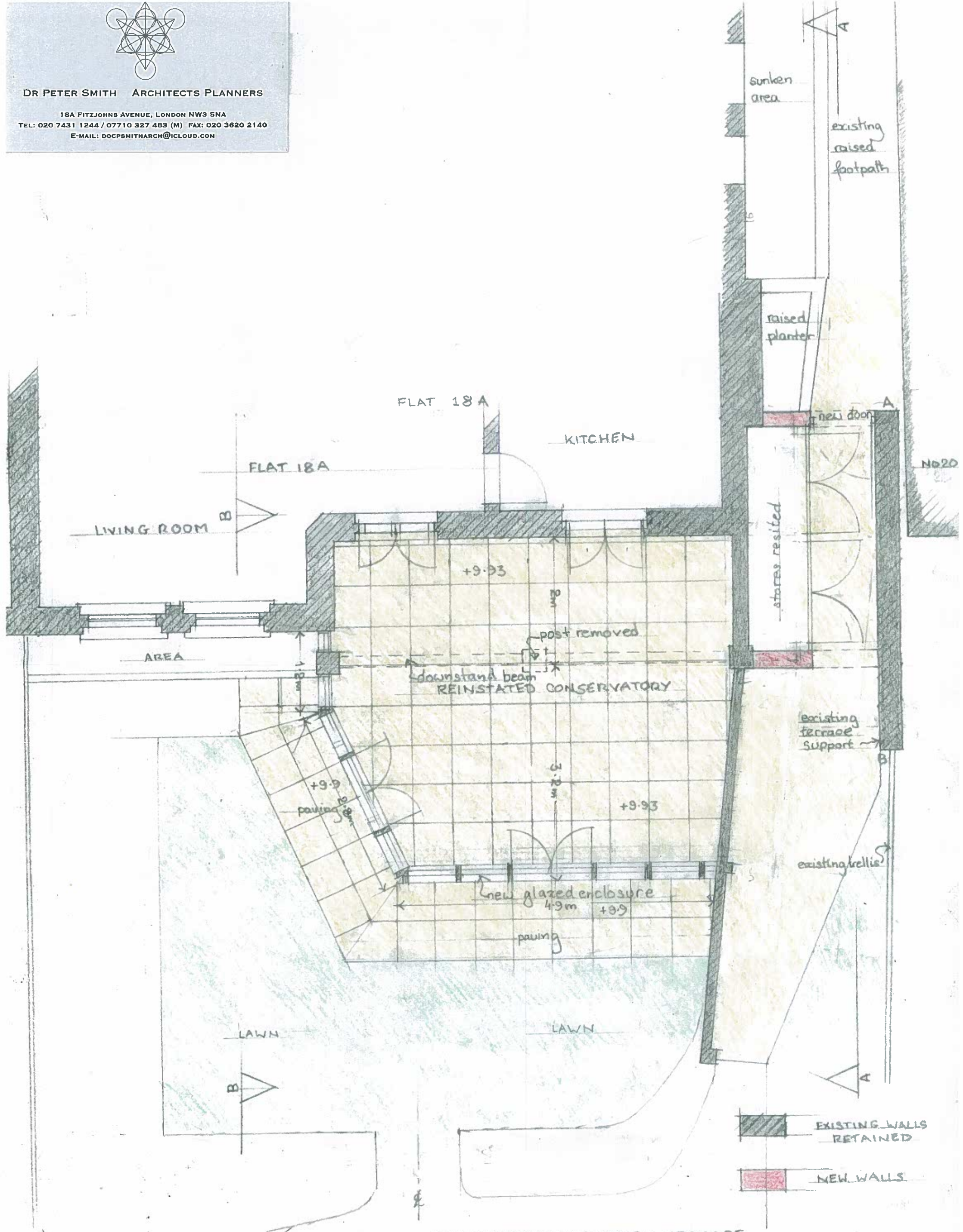
② 18 FITZJOHNS AVENUE ~ PROPOSED REINSTATEMENT OF GARDEN TERRACE
