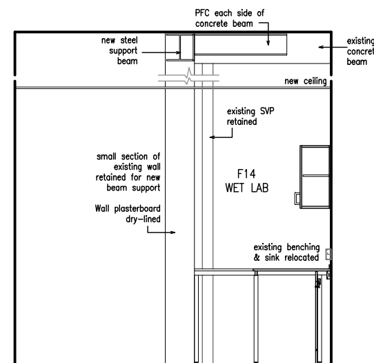
ELEVATION B - PROPOSED
