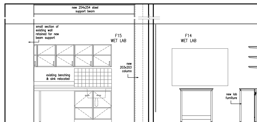
ELEVATION A - PROPOSED
