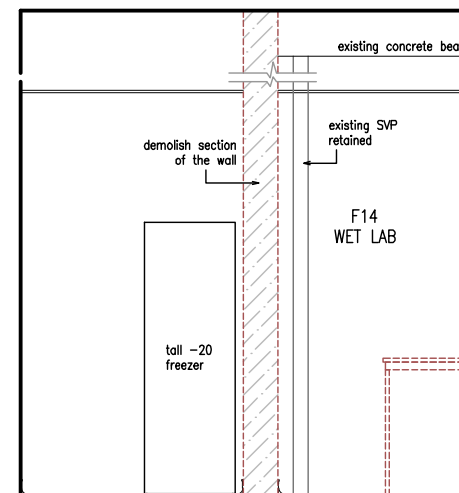
ELEVATION B - EXISTING
