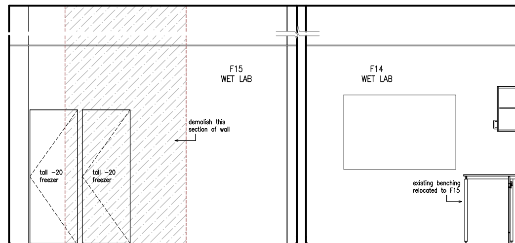
ELEVATION A - EXISTING
