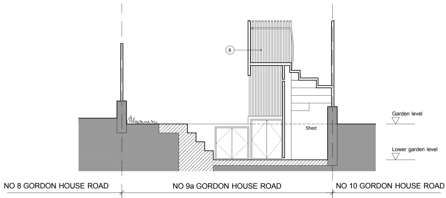
① Proposed section 1:50 @ A3
