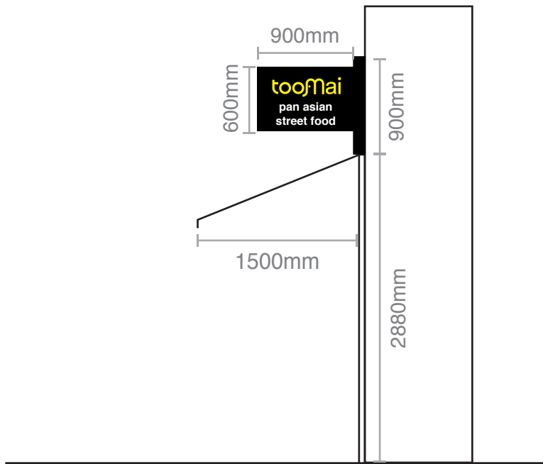
SIDE ELEVATION VIEW
