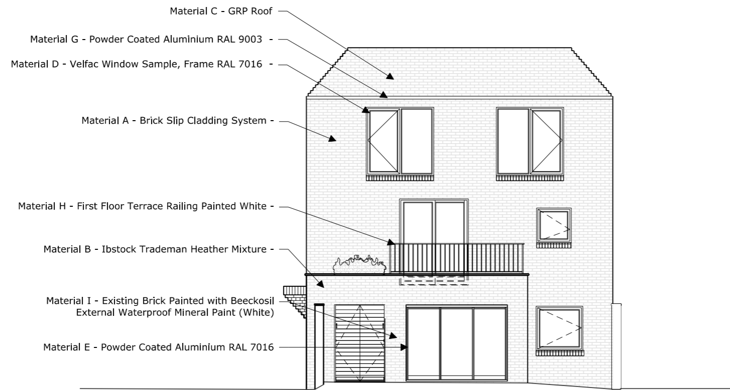
1 Proposed Elevation with no vegetation
