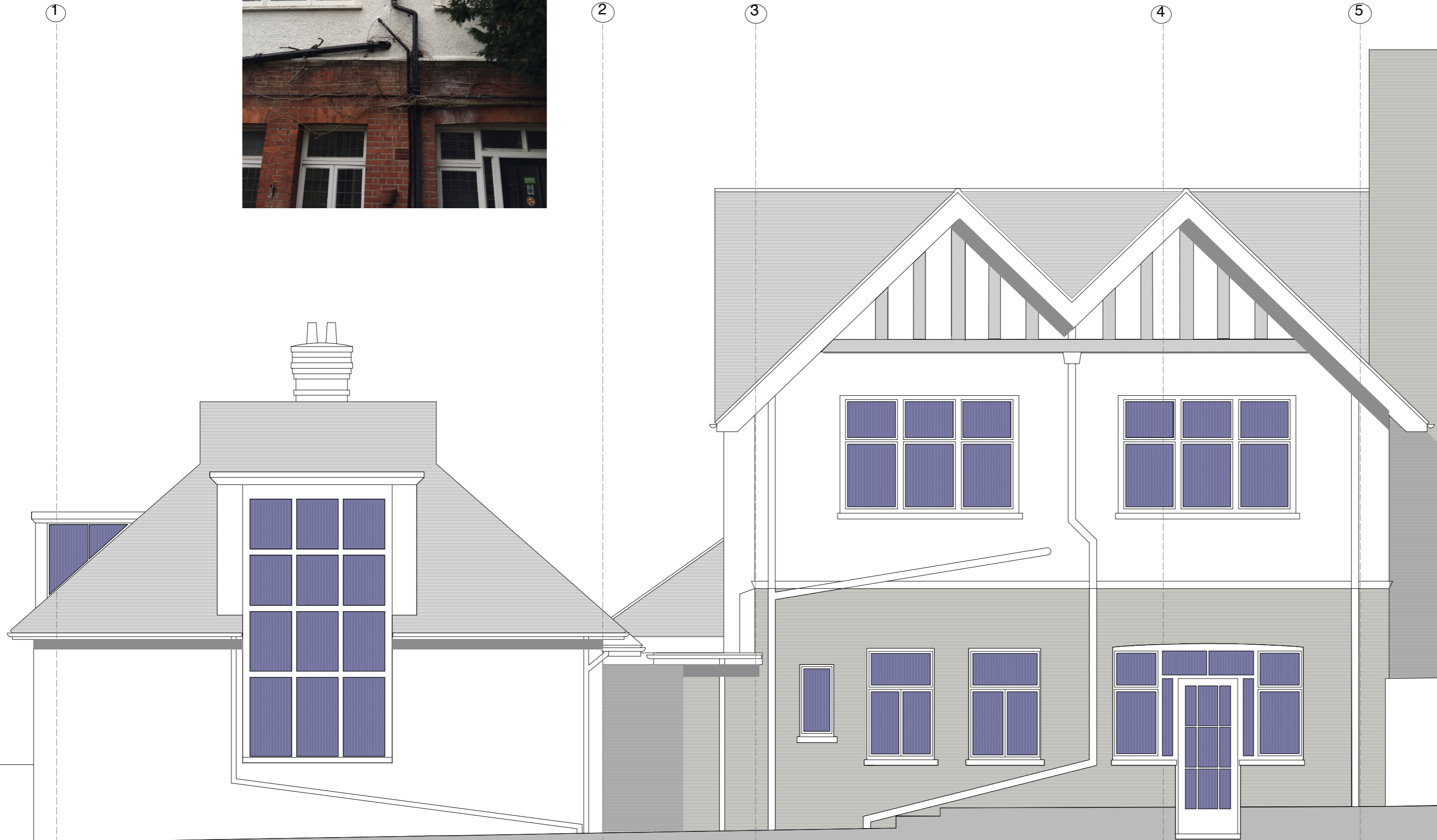
FRONT ELEVATION
