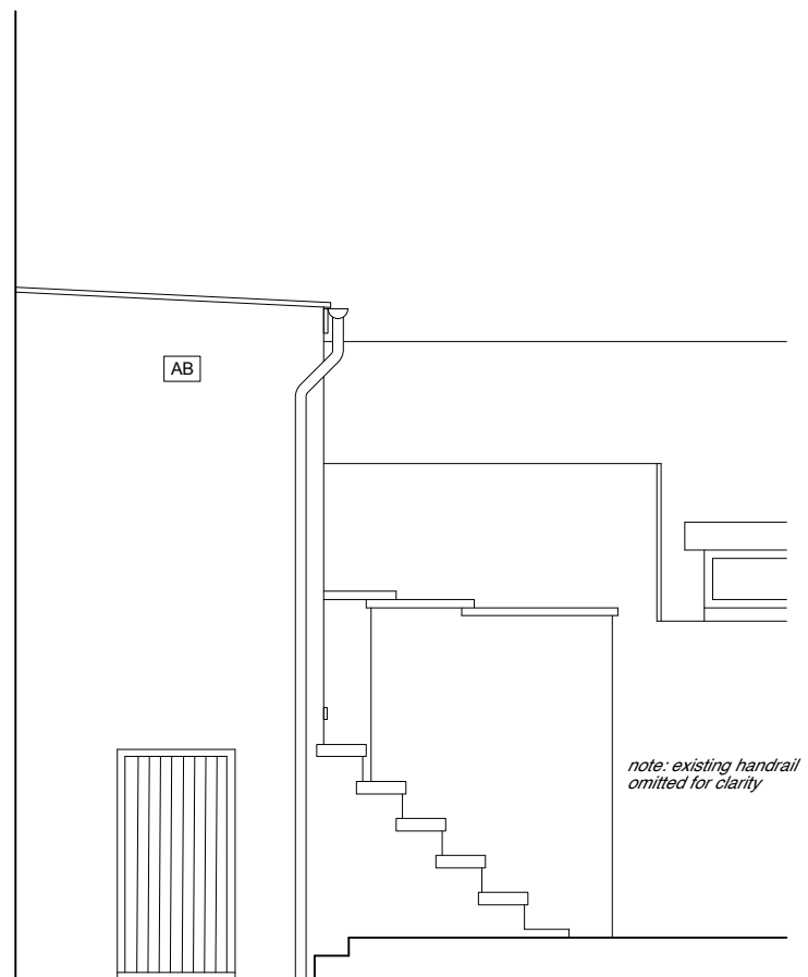
BACK EXTENSION SIDE ELEVATION (RAILINGS/BALUSTRADING OMITTED FOR CLARITY)
