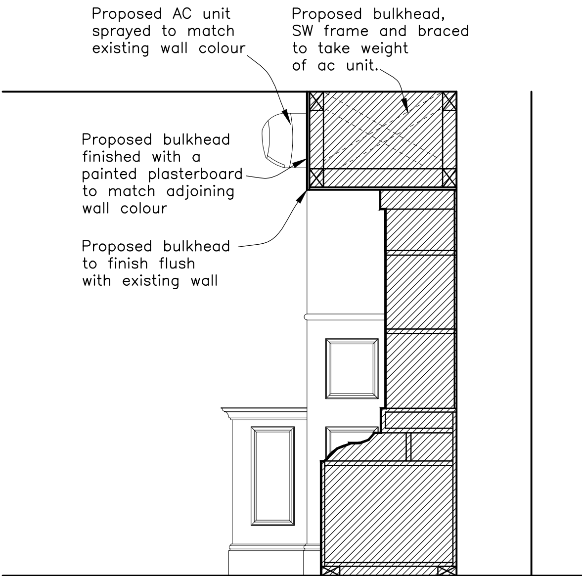
PROPOSED ELEVATION/SECTION C-C
