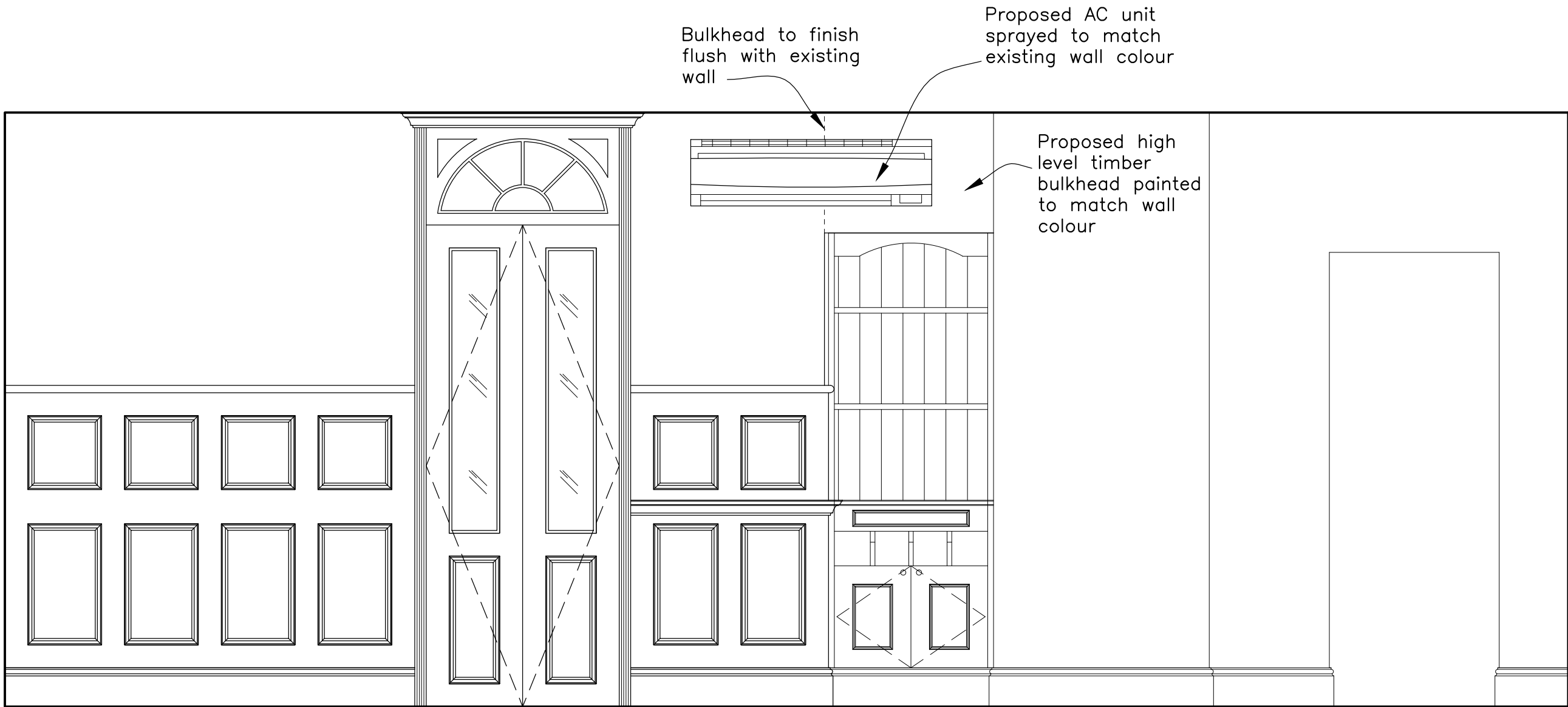
PROPOSED ELEVATION A-A
