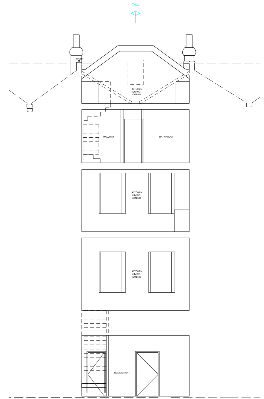
PROPOSED SHORT SECTION
