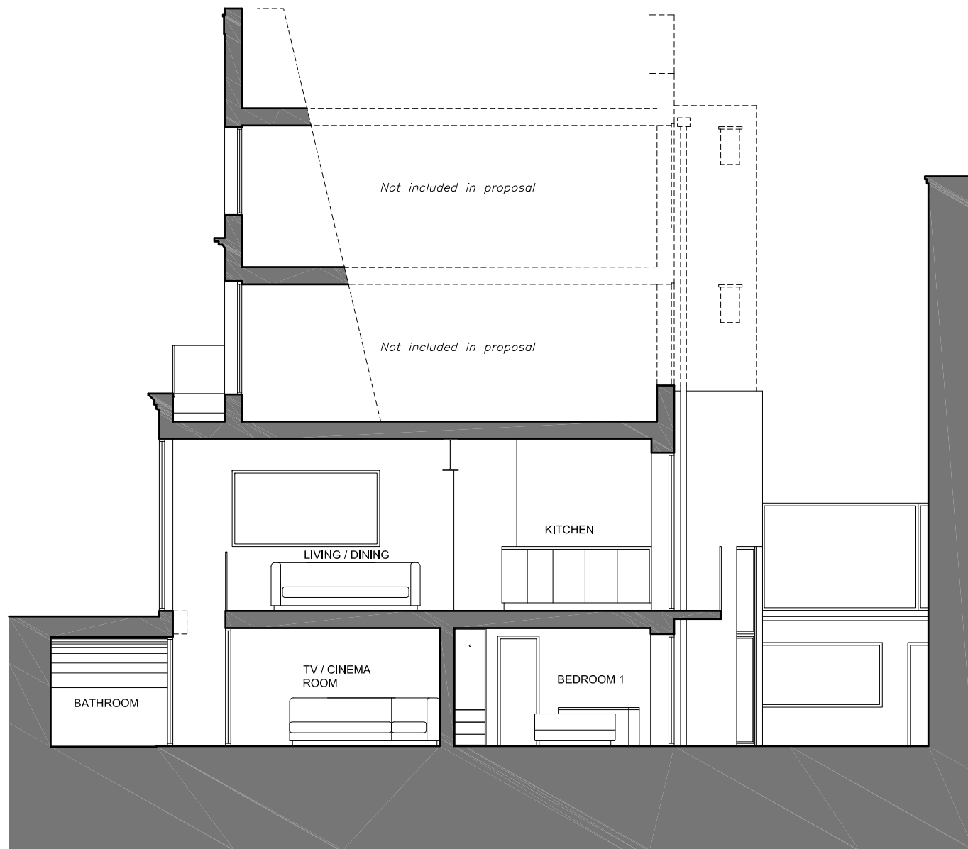
01 Section A
