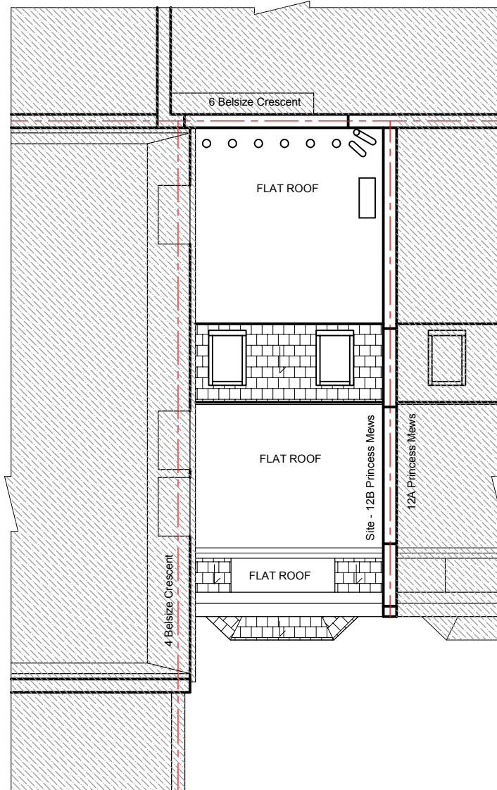
Existing Site Plan
