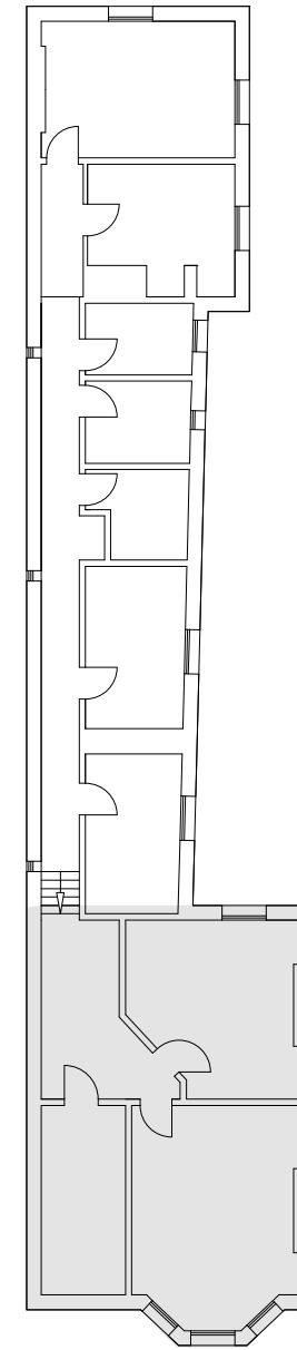
Plan of Apartment with area of development shaded 1:100@A1
