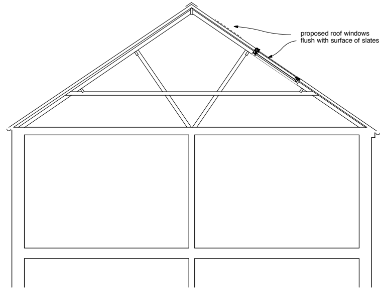
A-A Proposed Section
