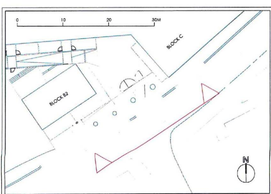
LOCATION MAP
