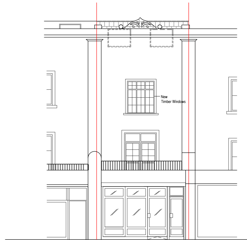
FRONT ELAVATION
