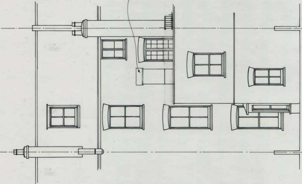
EXISTING REAR ELEVATION 1/50
