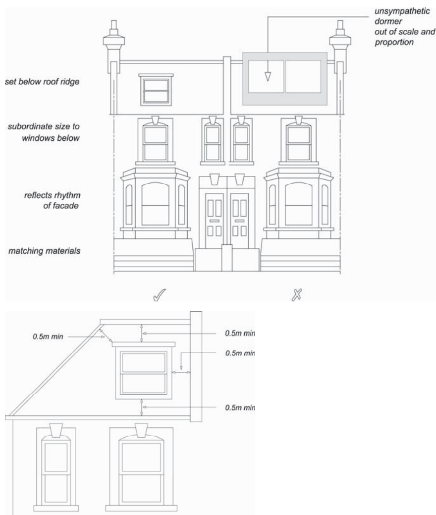
Figure 4. Dormer windows
