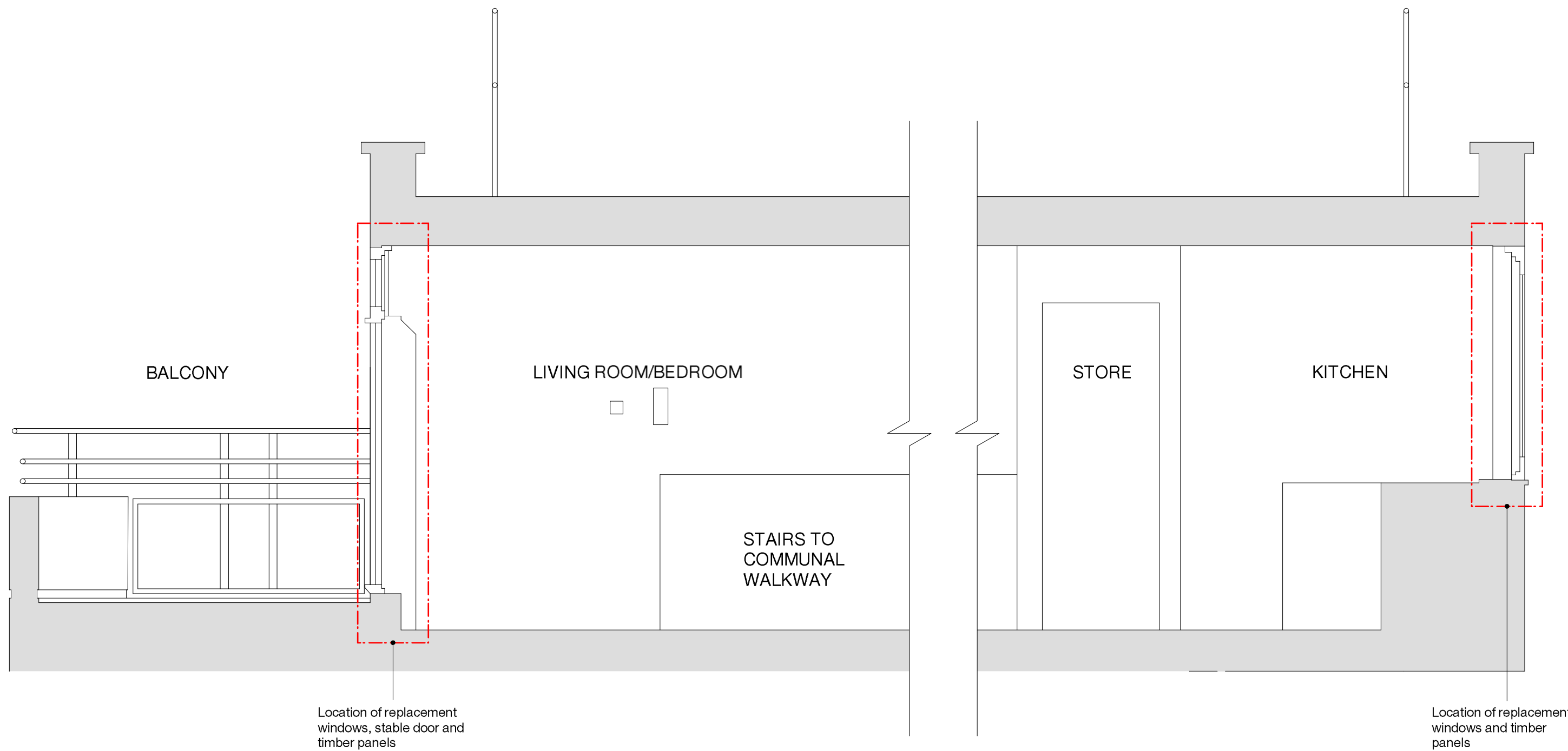
Proposed Typical Studio Flat Section AA - 1:25 Broadfield Lane
