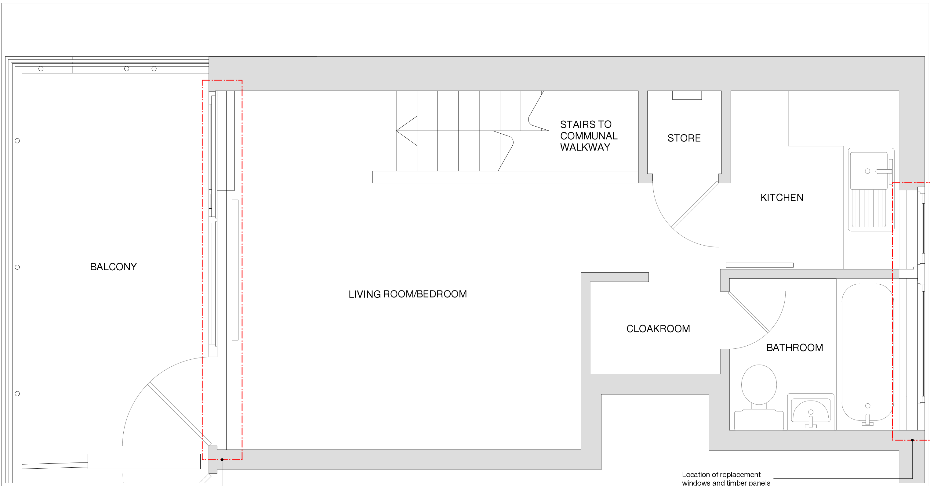
Proposed Typical Studio Flat Plan - 1:25 Broadfield Lane
