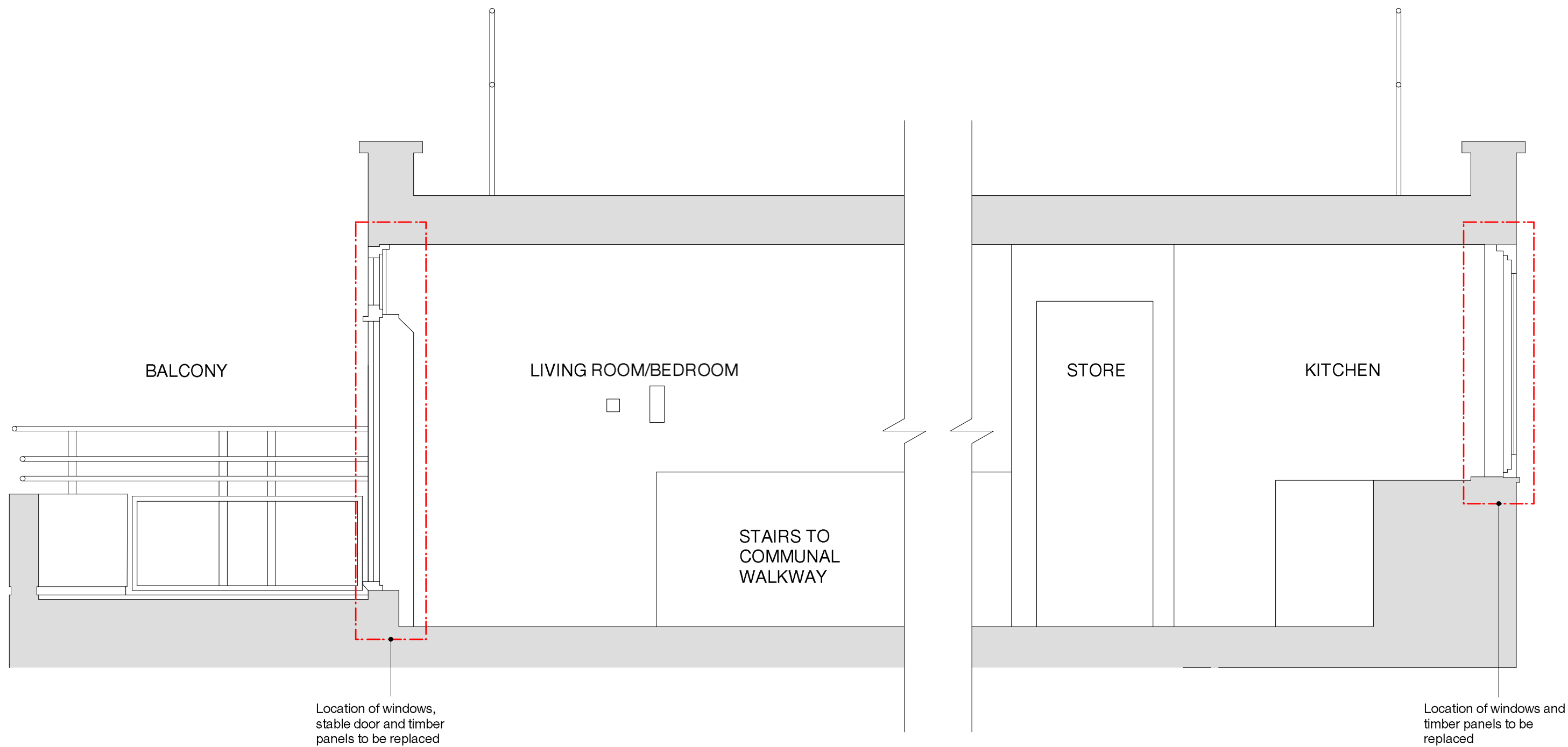
Existing Typical Studio Flat Section AA - 1:25 Broadfield Lane
