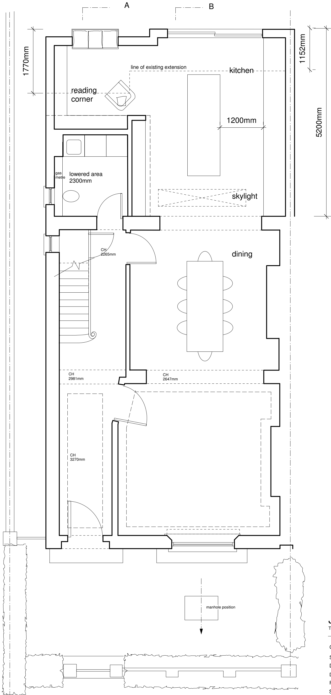
ground floor plan as proposed Option 3
