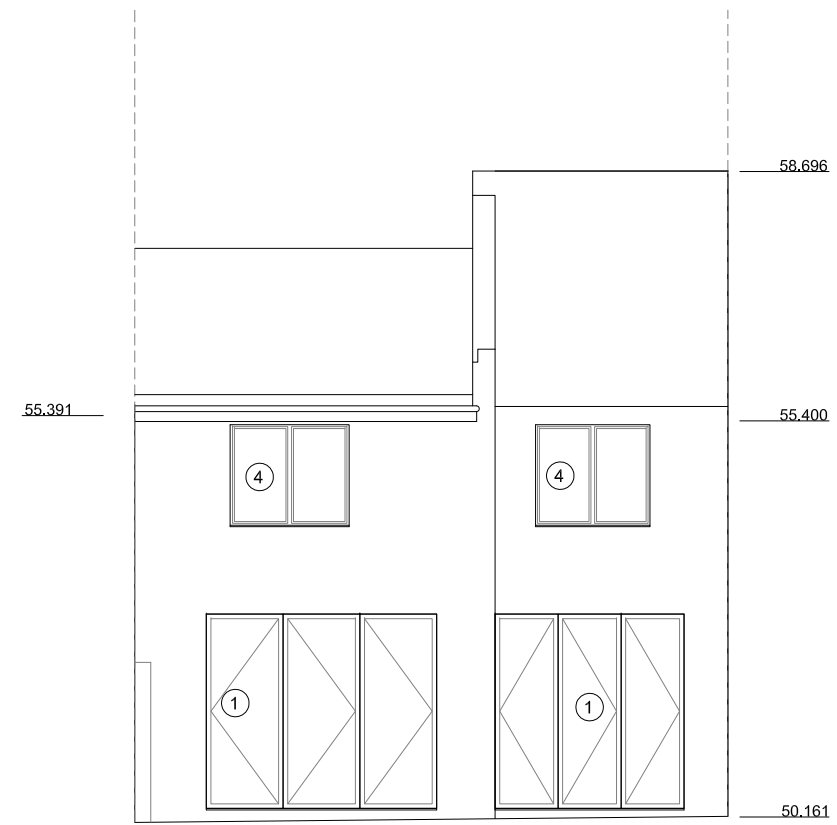
Elevation 4 Proposed
