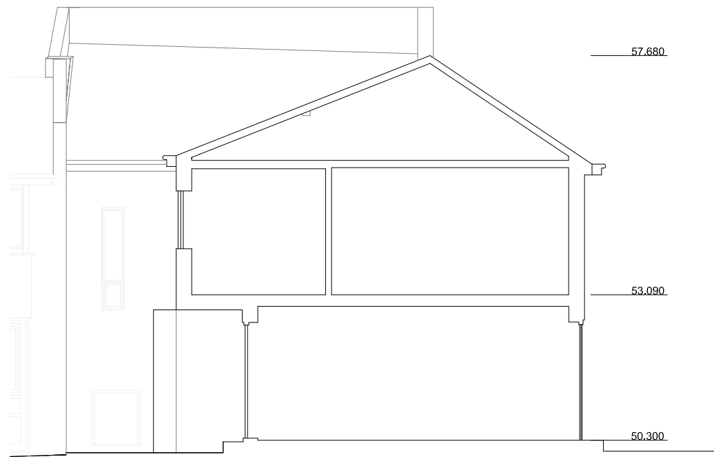
Section A - A Existing
