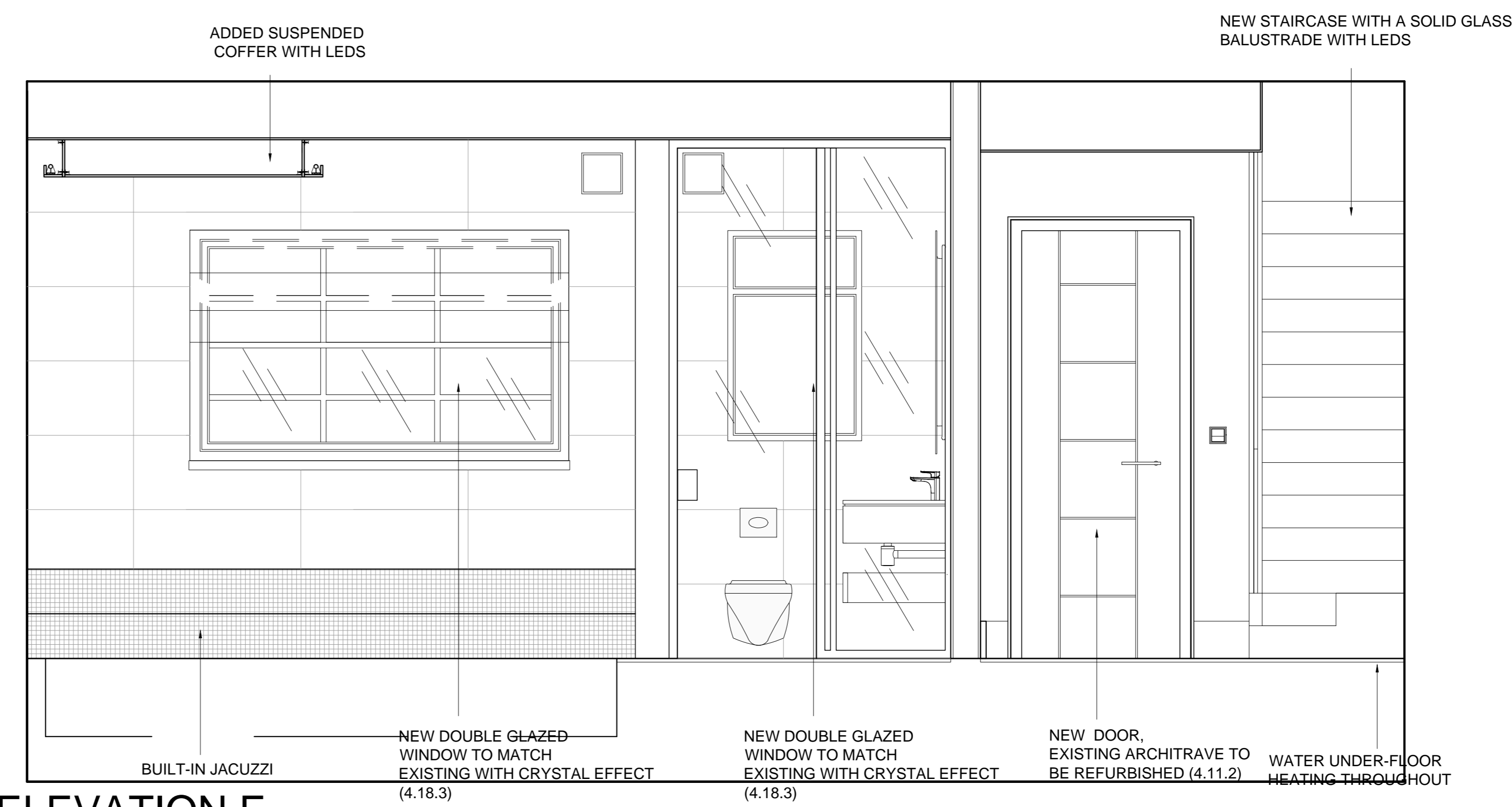
ELEVATION F
