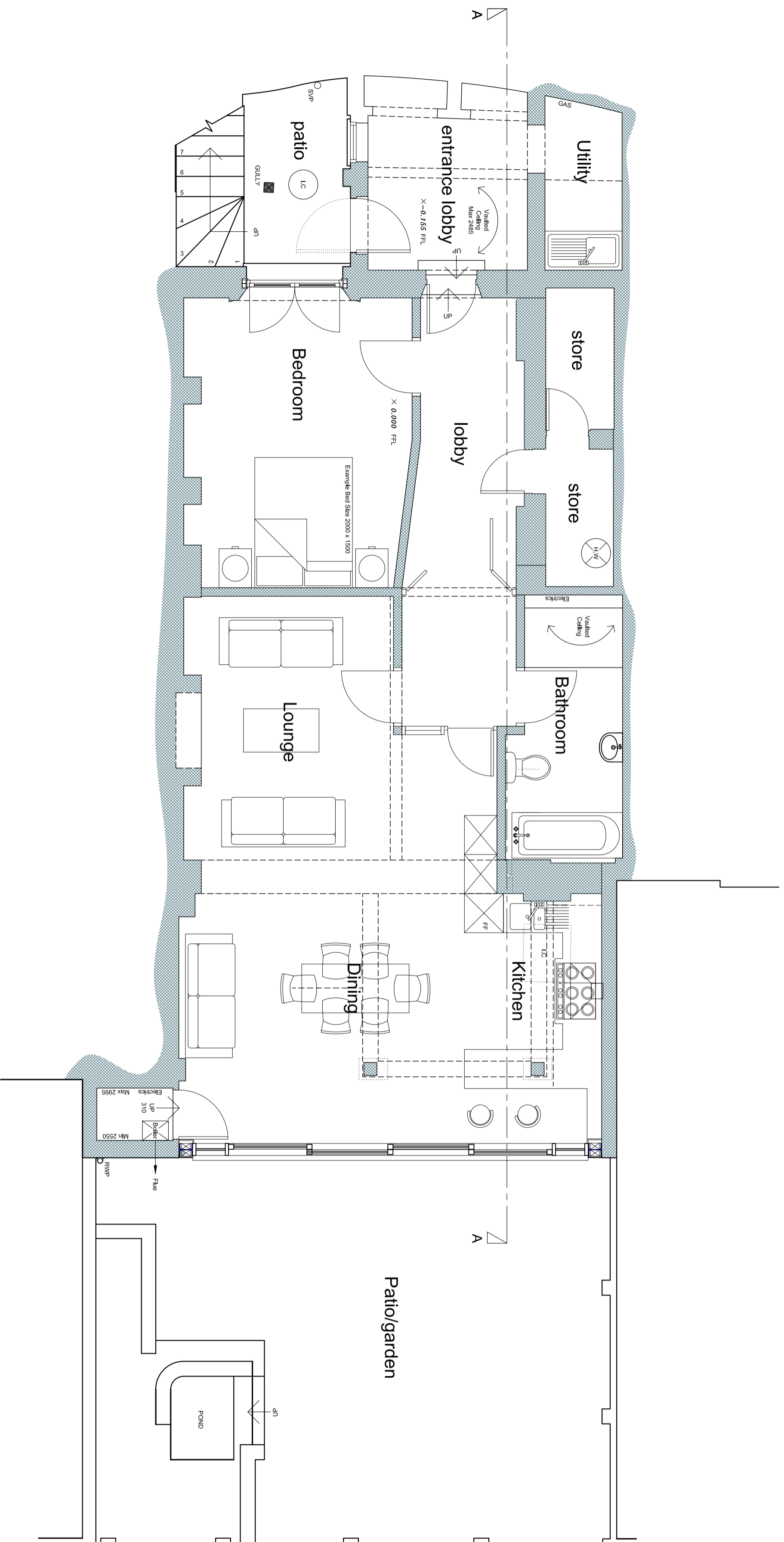
LOWER GROUND FLOOR PLAN
