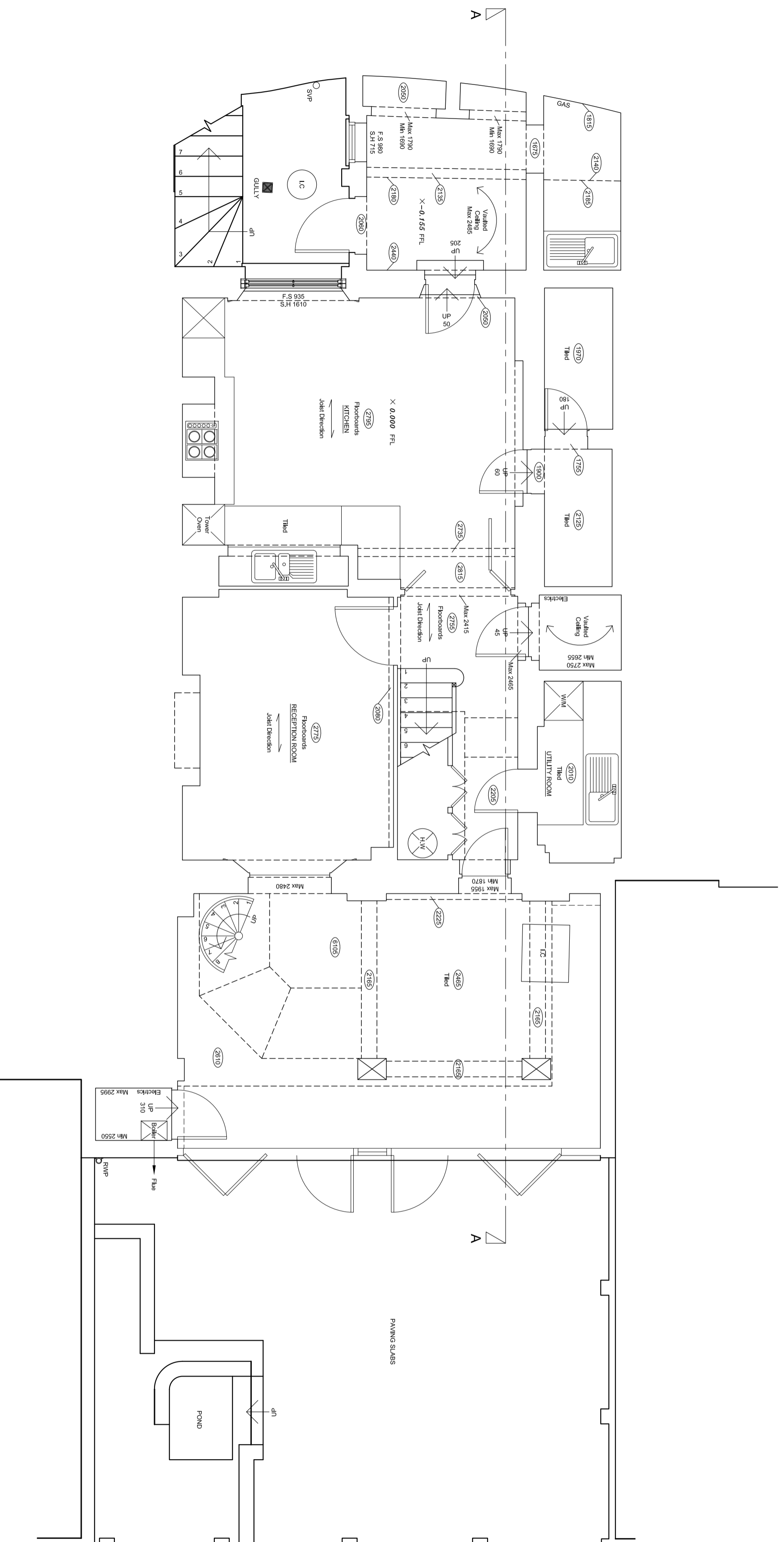
EXISTING LOWER GROUND FLOOR PLAN
