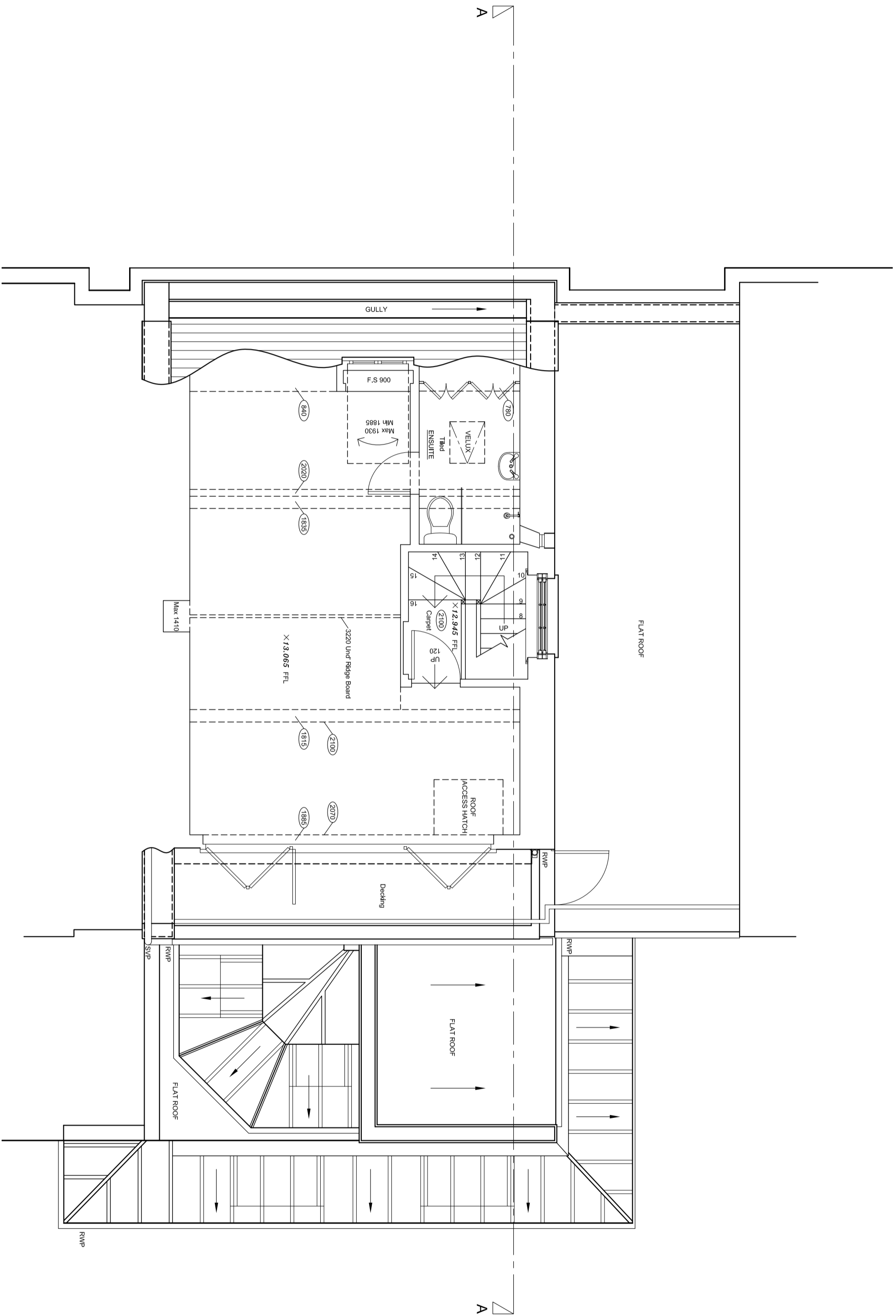
EXISTING THIRD FLOOR PLAN
